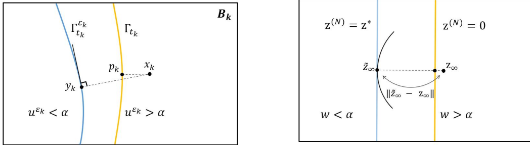
(a) Points x_k, y_k, p_k and interfaces \Gamma_{t_k}, \Gamma_{t_k}^{\varepsilon_k} inside the box B_k . (b) Points z_\infty and \tilde{z}_\infty and hyperplanes z^{(N)} = z^*, z^{(N)} = 0 .
