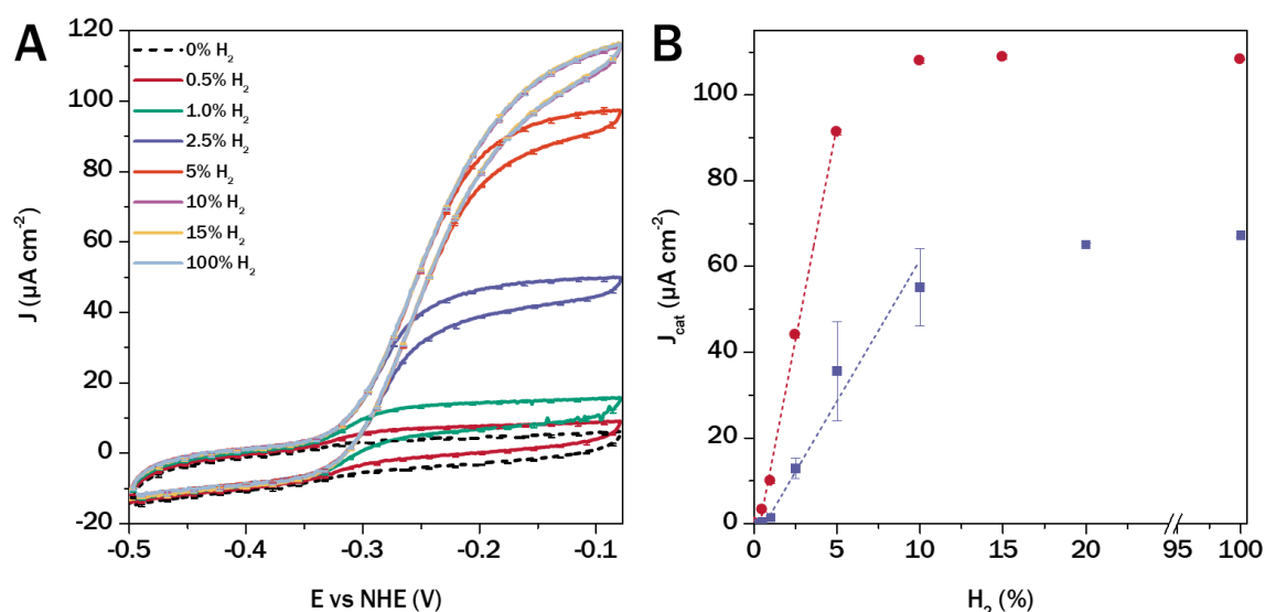
Figure 5. Calibration curves. (A) Averaged CVs of the Aa Hase modified RDE GC-MWCNT-NH 2 under various hydrogen content on RDE (2000 rpm); Phosphate buffer pH 7 (0.1M), V_{\text{MWCNT}} = 10 \mu\text{L} , V_{\text{enzyme}} = 5 \mu\text{L} , C_{\text{enzyme}} = 0.5 \mu\text{M} , adsorption for 30 mins at 4 °C; (B) Dependence of the catalytic current at -0.1 V (NHE) on the H 2 concentration without (blue squares) and with electrode rotation (red circles). Dashed lines indicate approximative linearity zone. Error bars represent standard deviations for four identical cycles.
