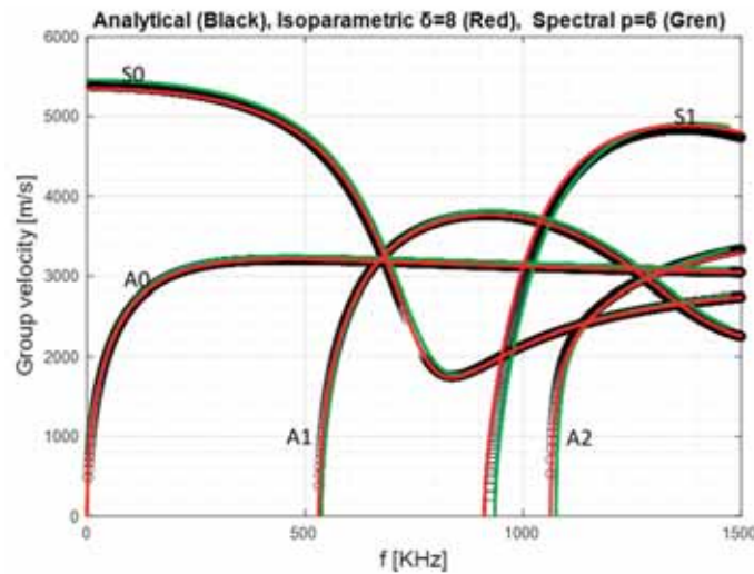
Figure 6. Group velocity dispersion curves calculated by SBFEM with isoparametric and spectral elements for a 3 mm-thick isotropic plate. Symmetric S_n and antisymmetric A_n ( n = 0, 1, 2, \dots ) modes.
