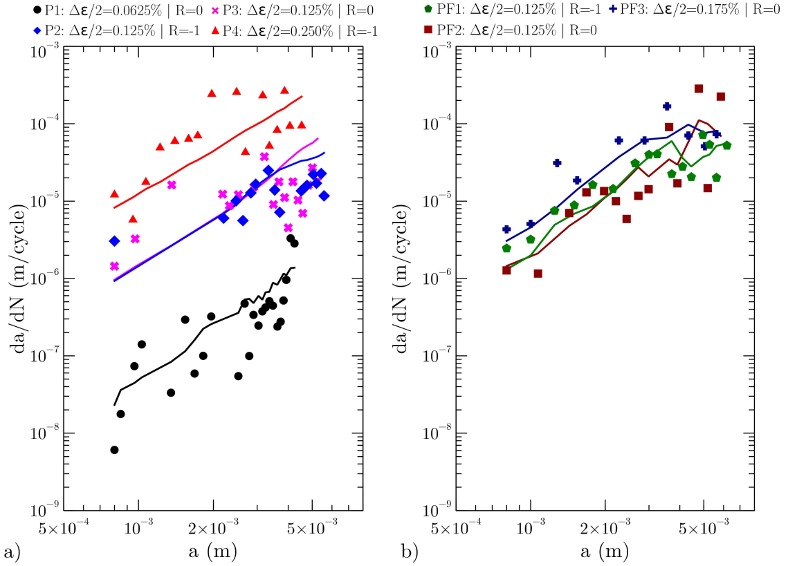
Figure 10: Fatigue crack growth rate as a function of the crack length for (a) porous material and (b) pore-free material. Markers symbolize experimental data, curves correspond to the model [30].
