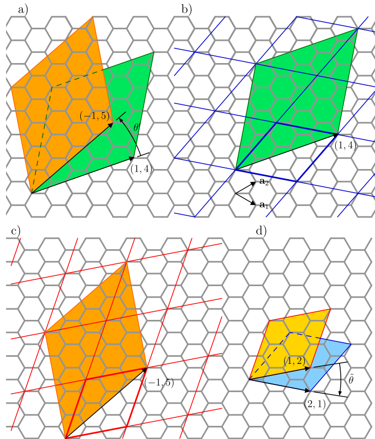
Figure 8: a) Construction of the moiré bilayer based on the (1, 4) supercell for the lower layer and the (−1, 5) for the upper layer. b) The lower supercell can be tessellated by the (2, 1) smaller supercell. c) The upper one is also a tessellation of the (1, 2) supercell. d) The angle of the “left-hand” small moiré is the same as that of the large non-primitive moiré \hat{\theta}_{\{2,1\}} = -\theta'_{\{1,4\}} .
