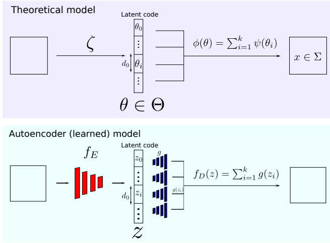
Fig. 1. Atomic autoencoder model. In this model, we consider an ideal latent space \Theta . Starting from an ideal latent code \theta \in \Theta , an ideal data point is generated by the sum of the same function \psi applied to k sub-blocks of \theta : \phi(\theta) = \sum_{i=1}^k \psi(\theta_i) , thus defining an atomic decoder architecture.
