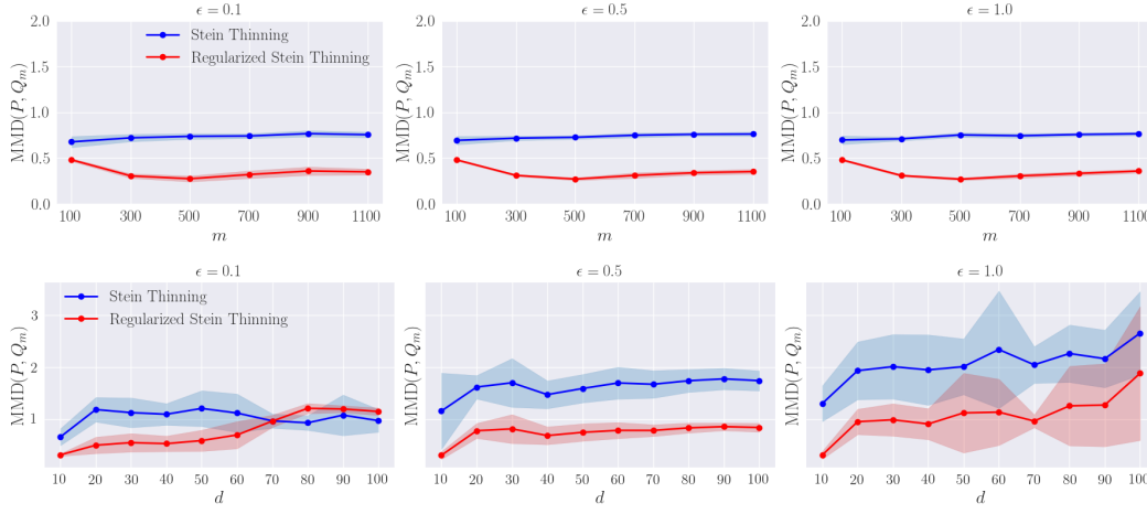
Figure 13: (Mixture of t-banana-shaped distributions, MALA) Graphs of the MMD distance with respect to the thinning size m (with d = 2 ) and with respect to d (with m = 300 ) for various step sizes \varepsilon .
