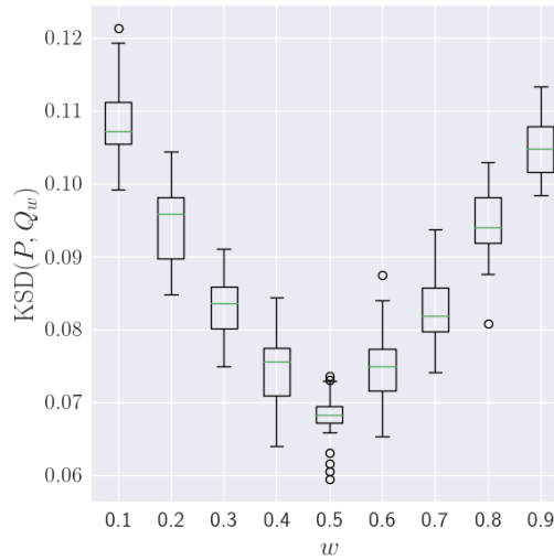
Figure 7: \text{KSD}(\mathbb{P}, \mathbb{Q}_w) for p as defined in Example 1 with \mu = 3, \sigma = 1, w_p = 0.2 , and q a truncation of p and with weight w . The KSD is estimated with n = 3000 and 30 repetitions for each w value.
