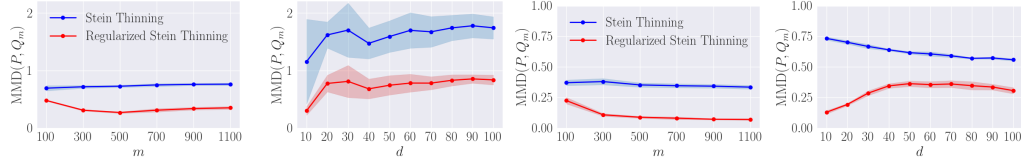
Figure 5: (MALA) Graphs of the MMD with respect to the thinning size m (for d = 2 ) and with respect to d (for m = 300 ). Left two panels: banana mixture. Right two panels: Gaussian mixture.
