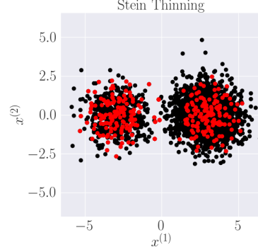
Figure 6: Illustration of Pathology I with the Gaussian mixture of Example 1 ( d = 2, \mu = 3, \sigma = 1, w = 0.2, n = 3000, m = 300 ). Initial particles are in black, and the Stein thinning output is red.
