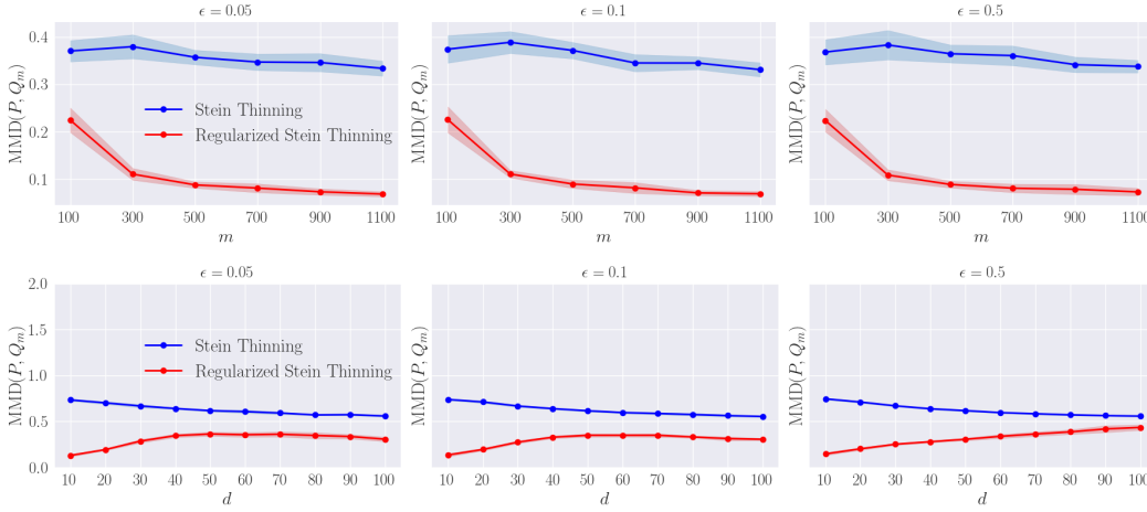
Figure 9: (Gaussian mixture, MALA) Graphs of the MMD distance with respect to the thinning size m (with d = 2 ) and with respect to d (with m = 300 ) for various step sizes \varepsilon .
