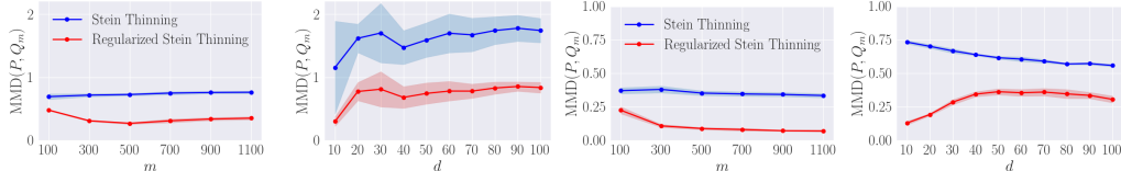
Figure 5: (MALA) Graphs of the MMD with respect to the thinning size m (for d = 2 ) and with respect to d (for m = 300 ). Left two panels: banana mixture. Right two panels: Gaussian mixture.
