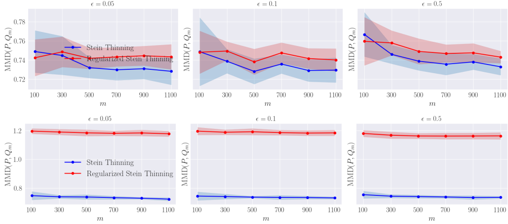
Figure 11: (Gaussian mixture, MALA) Graphs of the MMD distance with respect to the thinning size m (with d = 10 ) for various step sizes \varepsilon . For the first row, we set \lambda = 1/m^2 , and we observe that the effect of entropic regularization almost vanishes, since the performance is close to the original Stein thinning. For the second row, we set \lambda = 1/\log(m) , violating the convergence assumption, and resulting in bad thinned samples.
