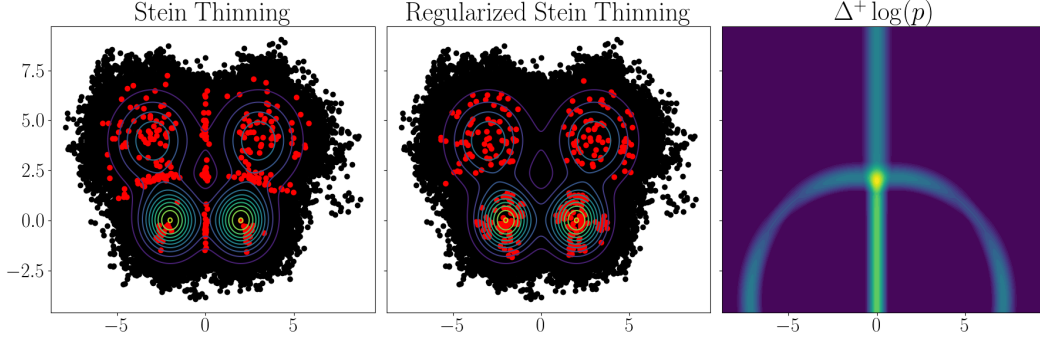
Figure 8: (Gaussian mixture with d = 2 , MALA) First two panels: solutions obtained with Stein thinning and regularized Stein thinning with contour lines of the target distribution. Last panel: heatmap of the Laplacian correction \Delta^+ \log(p) .
