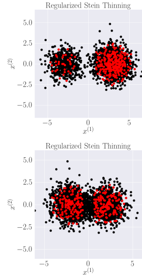
Figure 3: Pathologies fixed by the regularized Stein thinning.
