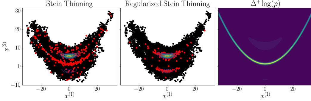
Figure 12: (t-banana-shaped mixture with d = 10 , MALA) First two panels: solutions obtained with Stein thinning and regularized Stein thinning with contour lines of the target distribution. Last panel: heatmap of the Laplacian correction \Delta^+ \log(p) for x^{(3)} = \dots = x^{(10)} = 0 .
