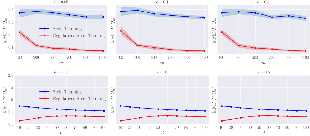
Figure 10: (Gaussian mixture, NUTS) Graphs of the MMD distance with respect to the thinning size m (with d = 2 ) and with respect to d (with m = 300 ) for various step sizes \varepsilon .
