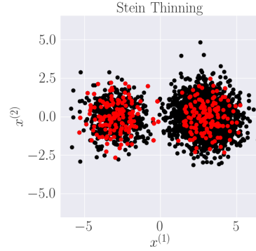
Figure 6: Illustration of Pathology I with the Gaussian mixture of Example 1 ( d = 2 , \mu = 3 , \sigma = 1 , w = 0.2 , n = 3000 , m = 300 ). Initial particles are in black, and the Stein thinning output is red.
