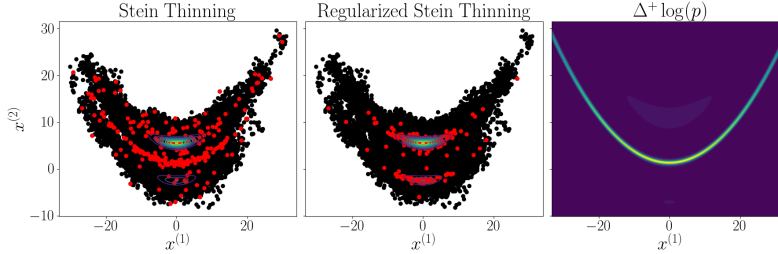
Figure 4: t-banana-shaped mixture ( d = 10 ). From left to right: solutions obtained with standard and regularized Stein thinning with contour lines of p , and heatmap of the Laplacian correction.
