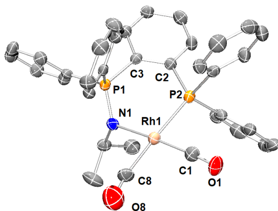
Figure 5. ORTEP plot of [\text{L}^{\text{N}}\text{Rh}(\text{CO})_2](\text{BF}_4) . Thermal ellipsoids are drawn at the 50% probability level. H atoms are omitted for clarity. Selected bond lengths (Å) and angles ( ^\circ ): Rh1–N1 2.118(3) , Rh1–P2 2.3086(11) , Rh1–C1 1.840(4) , C1–O1 1.134(4) , Rh1–C8 1.943(5) , C8–O8 1.073(5) , P1–N1 1.598(3) , P1–C3 1.821(4) , C2–C3 1.409(5) , C2–P2 1.832(4) , C1–Rh1–P2 87.77(13) , N1–Rh1–P2 93.95(9) , C1–Rh1–N1 176.74(16) , C8–Rh1–P2 175.99(13) , O1–C1–Rh1 176.3(4) , O8–C8–Rh1 171.1(4) .
