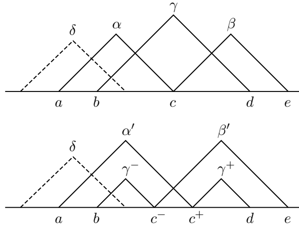
FIGURE 3. Replacing a configuration of one arc intersecting two adjacent arcs.
