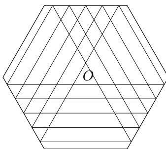
FIGURE 6. An area minimizing simple discrete disk (D, \mathcal{W}) of radius r = 5 where the topological disk D is a hexagon and the quasi wall system \mathcal{W} consists of straight lines.
