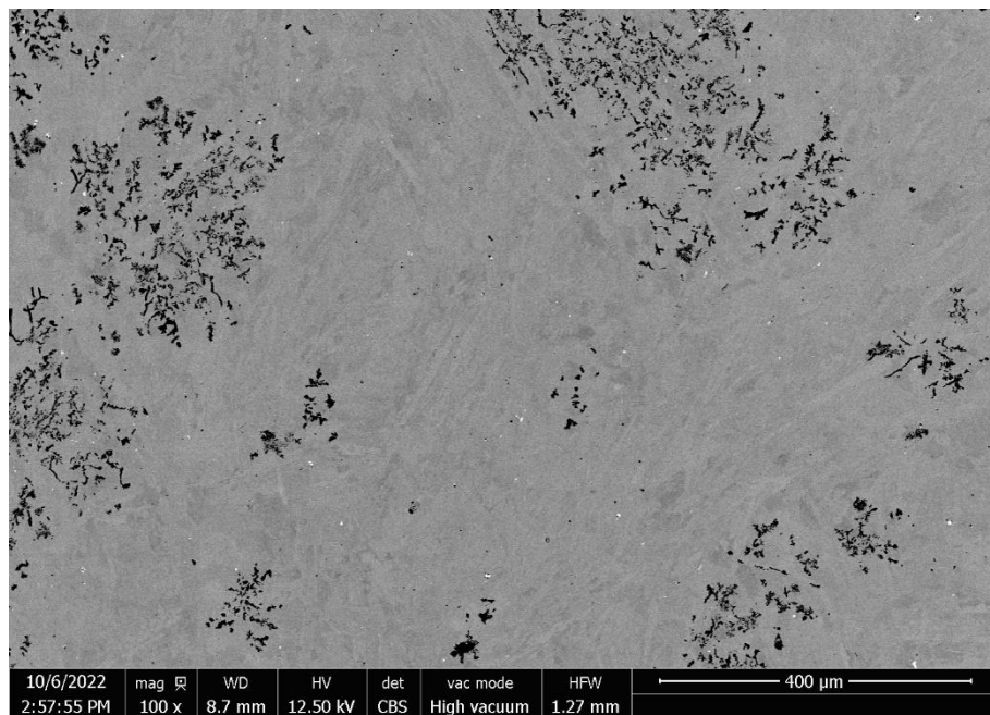
Figure B2. Low magnification SEM micrograph of the center of sample 19.5
