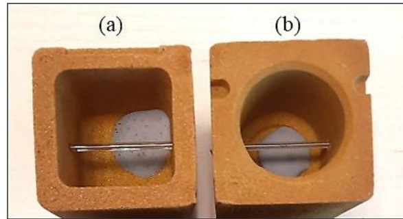
Figure 2. Upward view of the two different TA cups used in the present work: SQ cup (a) and RD cup (b). The grey patch at the bottom of the cavities is the Te-rich coating. The horizontal quartz tube protects the thermocouple whose junction is located in the middle of the cup. SQ cup cavities have a conical parallelepiped shape with a bottom base 35x35 mm, a upper base 37x37 mm and a height of 40 mm. The RD cups define a cylindrical volume with 34 mm in diameter and 40 mm in height.
