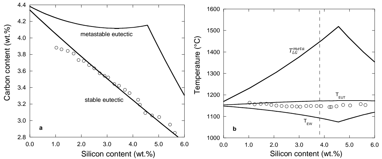
Figure 10. (a) plot of the composition of the stable and metastable eutectic lines calculated with TCFE8 with superimposed the composition of the investigated alloys (open circles). (b) Calculated temperatures T_{EUT} , T_{EW} and T_{LG}^{meta} (solid lines) and experimental T_{LA} temperatures for cup 5 (open circles). The dashed vertical line is positioned at 3.8 wt.% Si.
