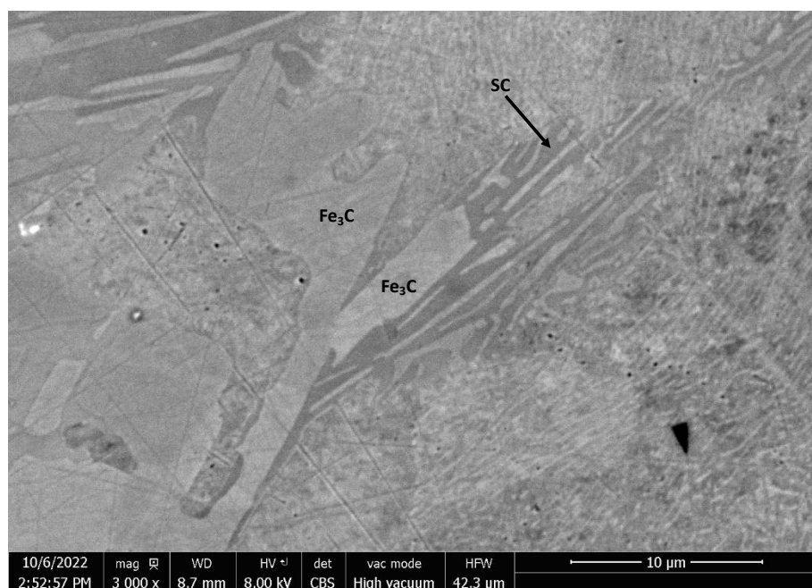
Figure B3. High magnification SEM micrograph of the matrix of sample 19.5.
