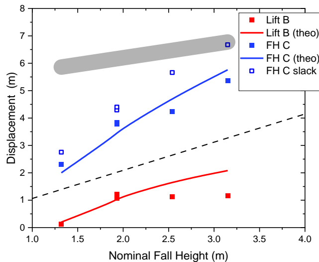
Fig. 2. Actual fall height of climber (blue) and belayer (red) as a function of nominal fall height. The dashed line represents the nominal fall height, the full lines are calculated using the equations derived by Leuthäusser [23]. The gray bar indicates ground-fall potential. (B = belayer; C = climber; FH = fall height)
