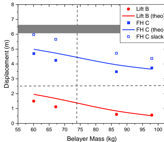
Fig. 5. Vertical displacement of climber (actual fall height) and belayer as a function of the belayer mass. Nominal fall height ( h_n = 2.54 m) and climber mass ( m_c = 73.7 kg) were kept constant. The vertical dashed line indicates m_c , the horizontal dashed line h_n . The full lines are calculated using the equations derived by Leuthäusser [23]. The gray bar indicates ground-fall potential
