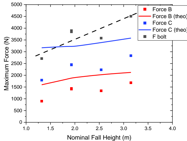
Fig. 3. Maximum forces the rope exerts on climber, belayer and bolt, respectively, as a function of nominal fall height. The full lines are calculated using the equations derived by Leuthäusser [23]
