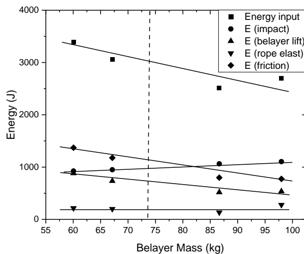
Fig. 7. Values of the various forms of energy involved in a fall as a function of belayer mass. The lines are guides to the eye
