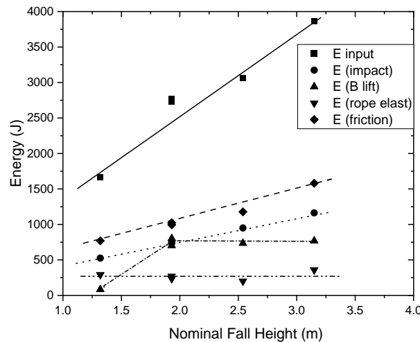
Fig. 4. Values of the various forms of energy involved in a fall as a function of nominal fall height. The lines are guides to the eye
