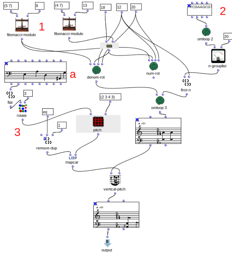
Figure 26: Patch generating Temporal Units starting from a DNA chain ([2]).
