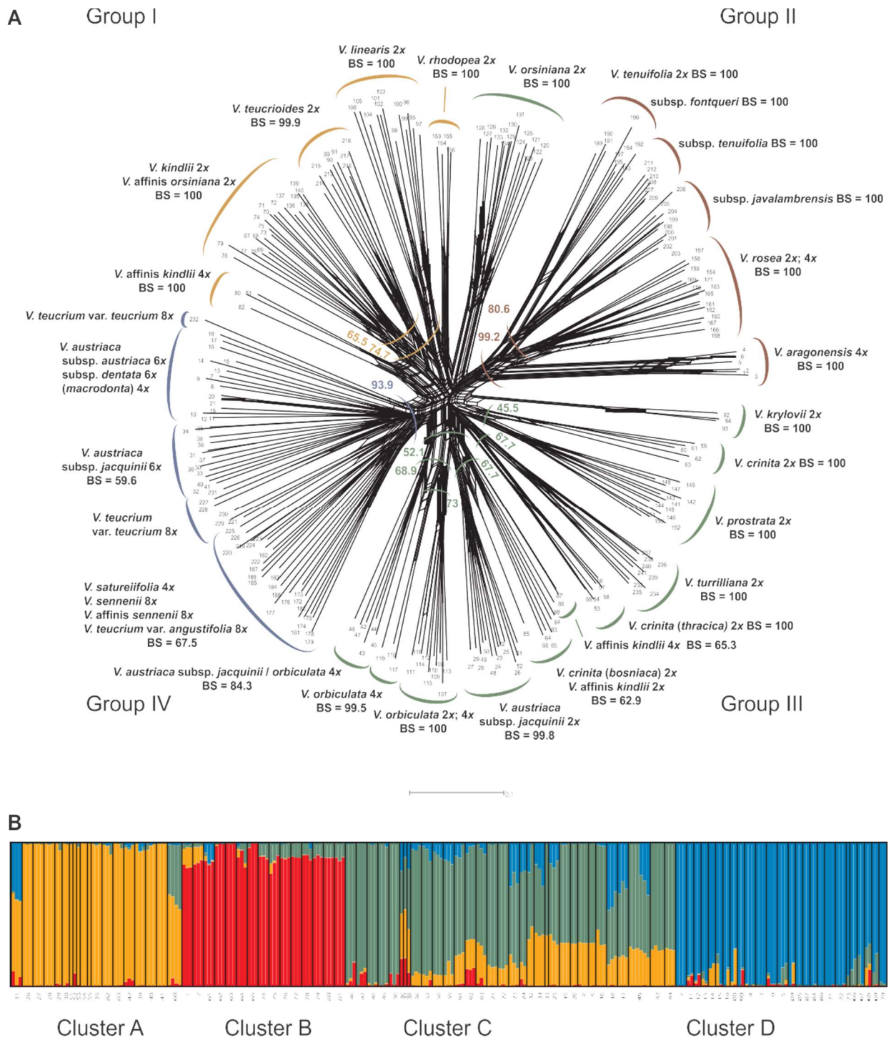
Fig. 2. (A) Neighbor-Net network based on 1127 AFLP scored fragments of 241 individuals of Veronica subsect. Pentasepalae using Jaccard's genetic distances. Individual codes are shown following Table S1. Arcs delimit taxa whose initial taxonomic determination and ploidy are shown. Range of colors of the arcs differentiates the four clusters identified by the Structure analyses. Bootstrap values (BS) > 50% are shown. (B) Bayesian clustering analyses based on the entire AFLP dataset. Four main clusters from a STRUCTURE analyses with K = 4 are represented by different colors. Black lines separate different populations which are indicated below the graph (population codes follow Table S1).
