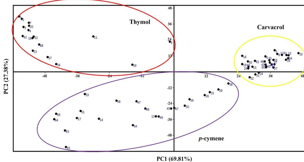
Fig. 2. PCA of the chemical composition of 68 EO samples from eight studied populations of O. grosii .
