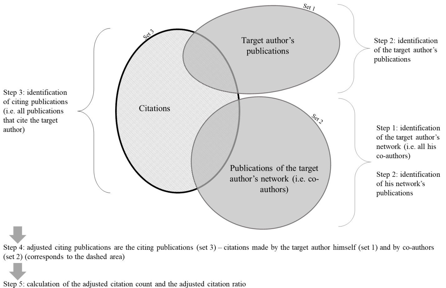
Fig. 1 Algorithm to compute the adjusted citation count metric. Note: the intersection between set 1 and set 3 represents the self-citations; the intersection between set 2 and set 3 represents the publications of the target author' network that cite at least one publication co-signed by the target author.
