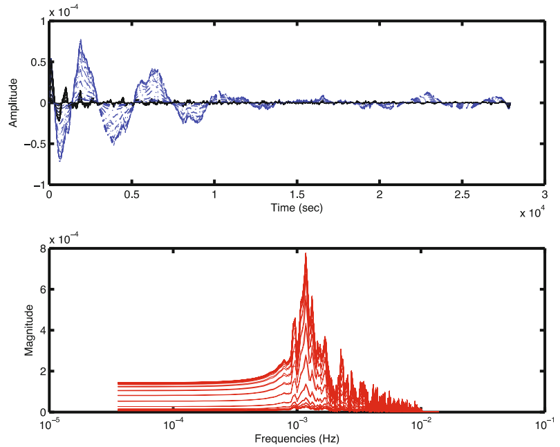
Fig. 5 Synthetic seismic signal ( blue detrended as to represent an instrumental record, black filtered [0.001,0.01] Hz) and corresponding frequency spectrum for the vertical component at all synthetic stations. Example from simulation #1
