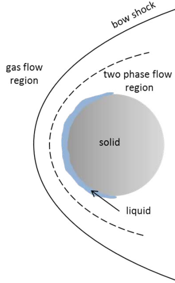
Figure 1: Description of the different phenomena occurring during the re-entry of a metallic debris.
