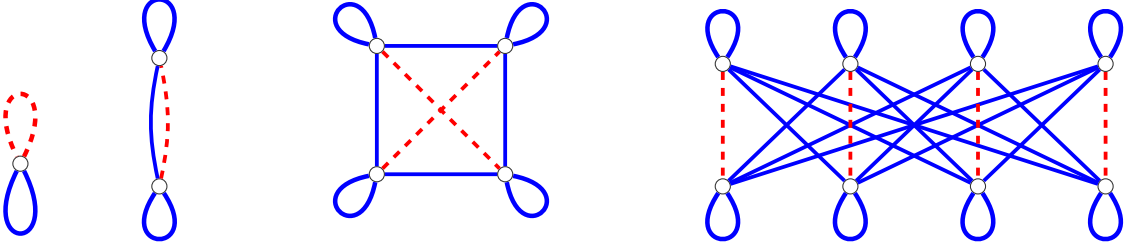
Figure 4: \mathcal{SPC}_d^o for d \in \{0, 1, 2, 3\}
