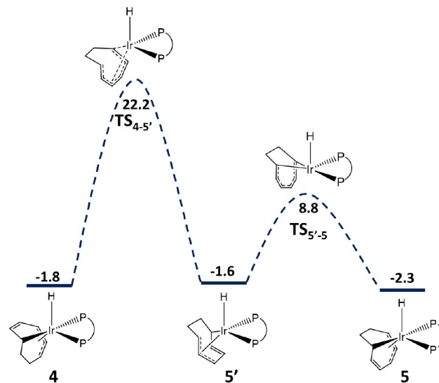
Figure 7. Gibbs-energy profile (in kcal mol -1 ) for the isomerisation of 4 to 5 by electronic rearrangement of the (1- \kappa -4,5,6- \eta^3 -C 8 H 10 ) ligand.
