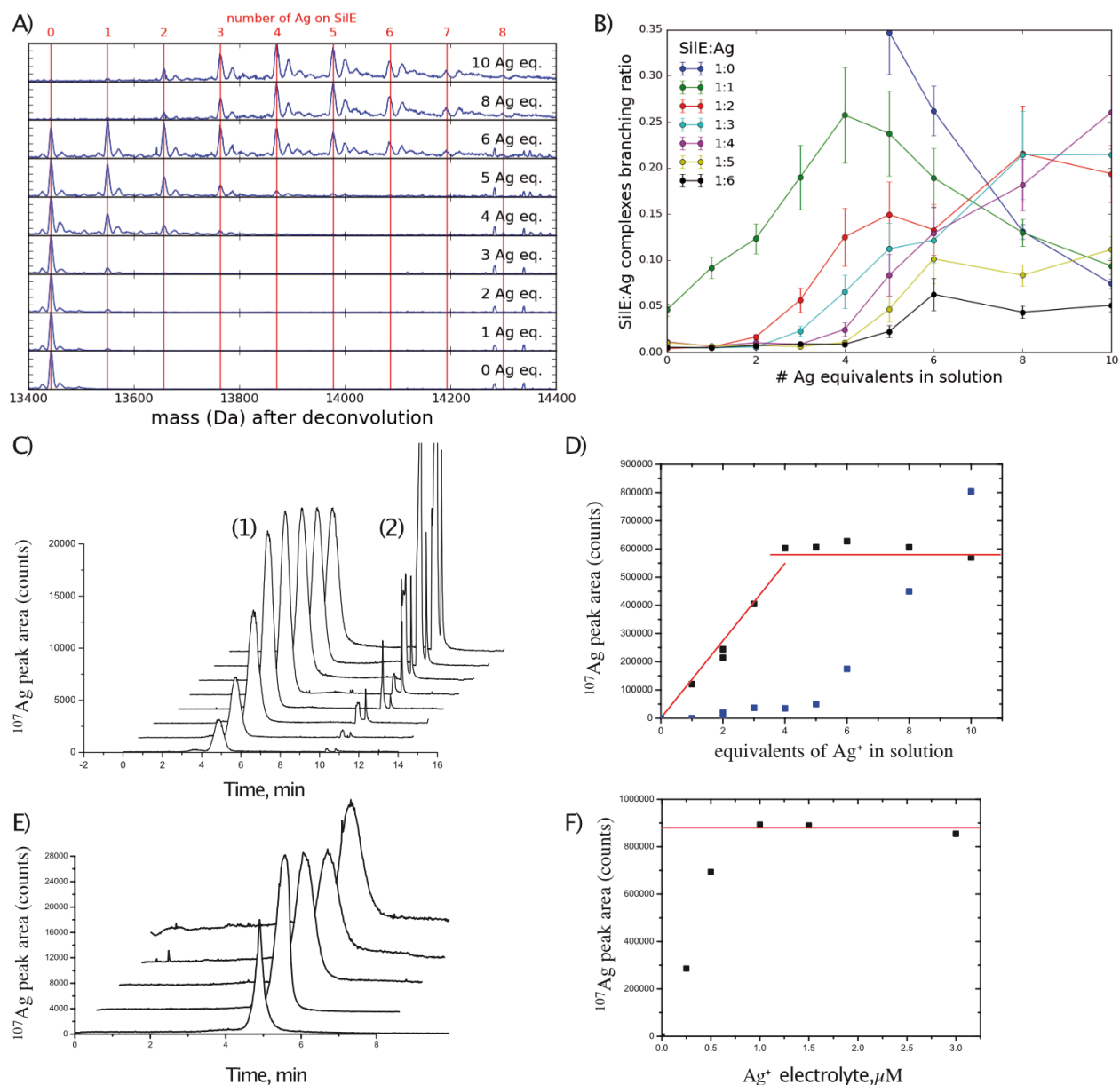
Figure 1. Stoichiometry of the Ag-SilE complex. A) Deconvoluted spectra, over the end of the elution band (in order to avoid chemical artefacts), of the 5 \mu\text{M} solutions of SilE and in presence of 1 to 10 molar equivalents of silver ions. The red lines represent the masses of the different stoichiometries [SiIE:nAg + ] complexes. B) Relative abundances or branching ratios of the different [SiIE:nAg + ] complexes as a function of the molar equivalents Ag + in solution. (C) Electropherograms obtained in CE-ICP-MS for 5 \mu\text{M} SilE and increasing Ag + concentrations in the sample for (1) [SiIE:nAg + ] complex and (2) sorbed Ag + released by HNO 3 . Electropherograms are shifted in 107 Ag signal intensity for sake of clarity, background signal is around 50 counts for all. (D) Peak areas measured from C) for Ag species as a function of the Ag + equivalents added in the sample for [SiIE:nAg] complex (black) and sorbed Ag + released by HNO 3 (blue). (E) Electropherograms obtained in CE-ICP-MS for 5 \mu\text{M} SilE and increasing Ag + concentrations in the electrolyte determined using CE-ICP/MS analyses. Electropherograms are shifted in 107 Ag signal intensity for sake of clarity. (F) Peak areas measured from E) for [SiIE:nAg] complex as a function of the Ag + concentration in the electrolyte.
