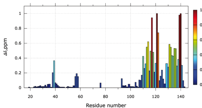
Figure 3. Silver binding sites. CSP observed at the end of the titration for 6 \text{Ag}^+ equivalent on a 140 \mu\text{M} ^{15}\text{N} -SiIE (20 mM MES buffer pH 6.8 and 20 mM NaF). Residues 59-92 (except 76) are missing due to the large signal broadening in ^1\text{H} - ^{15}\text{N} HSQC spectra.
