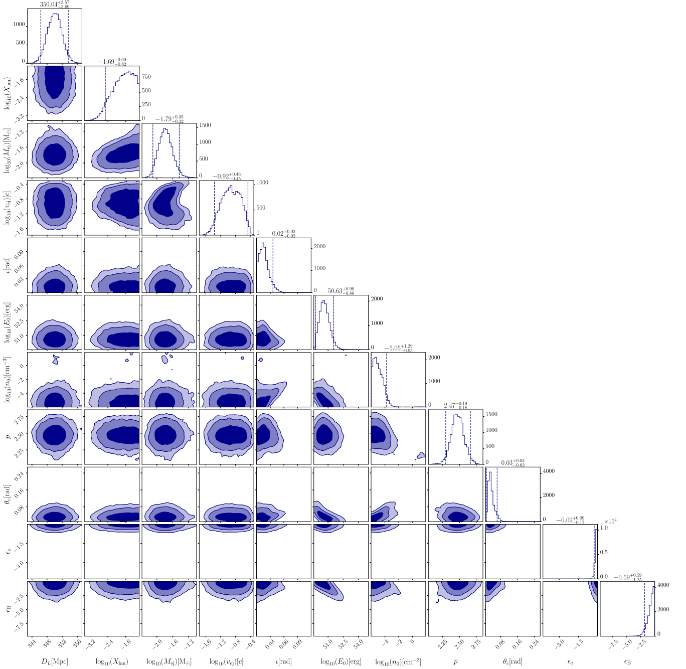
Figure B1. Corner plot for BNS-GRB- M_{\text{Kasen}}^{\text{top}} with a narrow Gaussian luminosity distance prior centred around 350 Mpc, in which we show the inferred parameters at 68 per cent, 95 per cent, and 99 per cent confidence (shadings from light to dark). For the 1D posterior probability distributions, we report the median values and show the 90 per cent confidence intervals as dashed lines.
