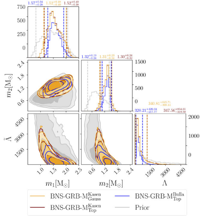
Figure 4. Component masses m_{1,2} and the dimensionless tidal deformability \Lambda based on our inference results of BNS-GRB- M_{\text{Gauss}}^{\text{Kasen}} (orange), BNS-GRB- M_{\text{Top}}^{\text{Kasen}} (red), and BNS-GRB- M_{\text{Top}}^{\text{Bulla}} (blue). Different shadings mark the 68 per cent, 95 per cent, and 99 per cent confidence intervals. For the 1D posterior probability distributions, we give the 90 per cent confidence interval (dashed lines) and report median values above each panel. Grey shaded areas give the prior probability regions.
