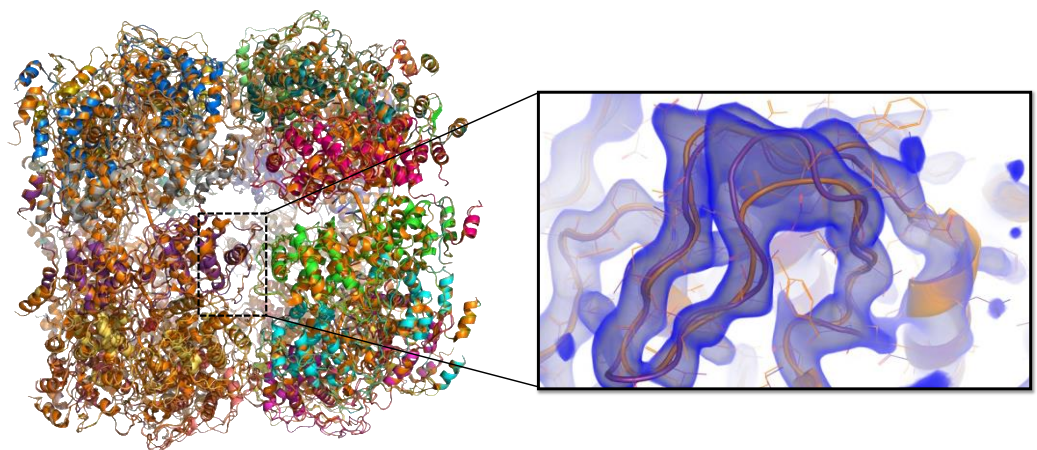
Figure 5. Re-refinement of the circular polymeric N_{11} -RNA complex crystal structure. The different N subunits of the re-refined model are shown in cartoon representation with different colors for each chain and superimposed onto the original model (PDB ID 2GTT, shown in orange). The close-up view shows an excerpt of the region that was rebuilt (in orange), with the experimental 2Fo-Fc map shown in volume representation in blue and contoured at 1\sigma (drawn with PyMOL).
