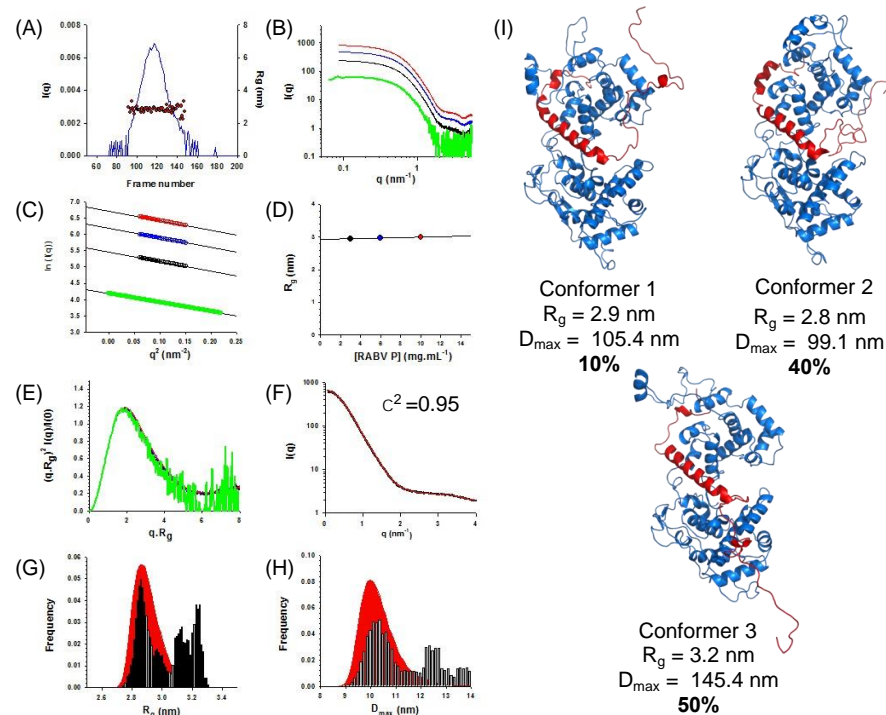
Figure 3. SAXS and SEC-SAXS of RABV N Δ23 0 -P 68 core complex. (A) SEC-SAXS elution profile and R g across the elution peak; 50 \mu L of the N Δ23 0 -P 68 sample were injected onto a Superdex 200 column and monitored on-line by SAXS. The black line shows the intensity at zero angle (I 0 ), which is proportional to both the MM and concentration. The red dots indicate the values of the radius of gyration calculated from the Guinier approximation at the different time intervals. (B) SAXS profiles at different protein concentrations. SAXS profiles were recorded in batch mode at 3 mg·mL -1 (in black), 6 mg·mL -1 (in blue), and 11 mg·mL -1 (in red). The curve in green was obtained by averaging the individual profiles recorded throughout the SEC elution peak shown in Panel (A). (C) Guinier plots at different protein concentrations. Same color scheme as in panel (B). (D) R g at different protein concentrations. The R g value were calculated from the Guinier plot (panel (C)) for the profiles recorded in batch mode. (E) Dimensionless Kratky plots at different protein concentrations. Same color scheme as in panel (B). (F) Merged curve and conformational ensemble modeling by the ensemble optimization method (EOM). The black line shows the scattering profile obtained by merging segments of the profiles obtained at different protein concentrations (panel (B)). The red line shows a back-calculated scattering curve for a selected ensemble of three conformers measured in different proportions and shown in panel (I) ( \chi^2 = 0.95 ). (G) R g distribution. The red area shows the R g distribution calculated for the initial ensemble of conformers, whereas the black bars show the R g distribution of the selected ensemble that fit the experimental SAXS data (panel (F)). (H) D max distribution. The red area shows the D max distribution calculated for the initial ensemble of conformers, whereas the black bars show the D max distribution of the selected ensemble that fit the experimental SAXS data. (I) Representative ensemble of conformers. N is shown in blue and P 68 including the eight C-terminal residues of the linker and His-tag are shown in red (cartoon representation).
