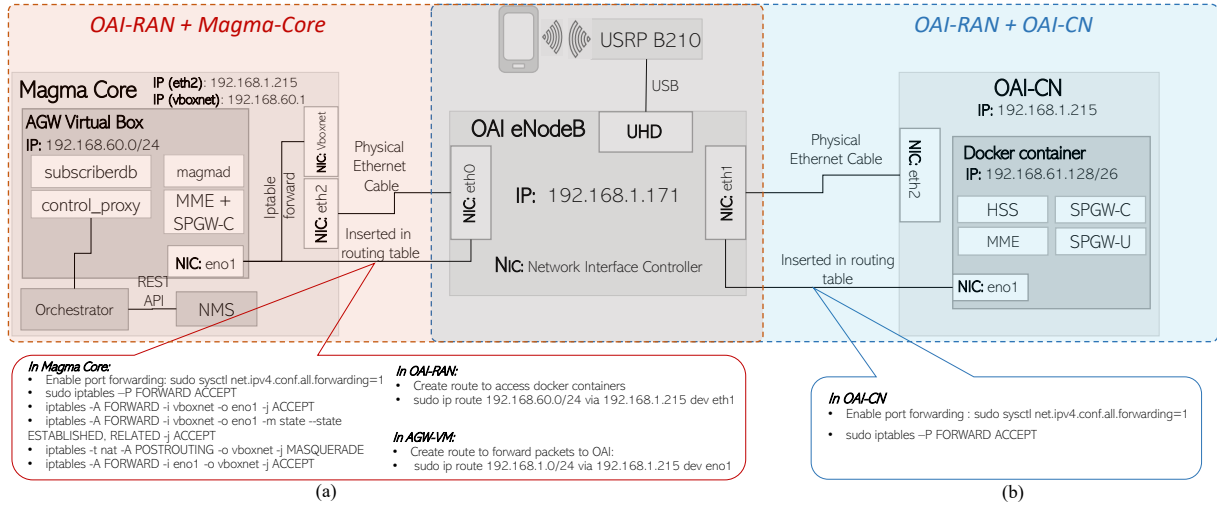
Figure 1. Architecture of deployed testbed. (a) the red box denotes Smartphone \leftrightarrow OAI – RAN+Magma – CN , and (b) the blue box shows Smartphone \leftrightarrow OAI – RAN+OAI – CN . The intersection of two boxes depict OAI-RAN common to both scenarios.
