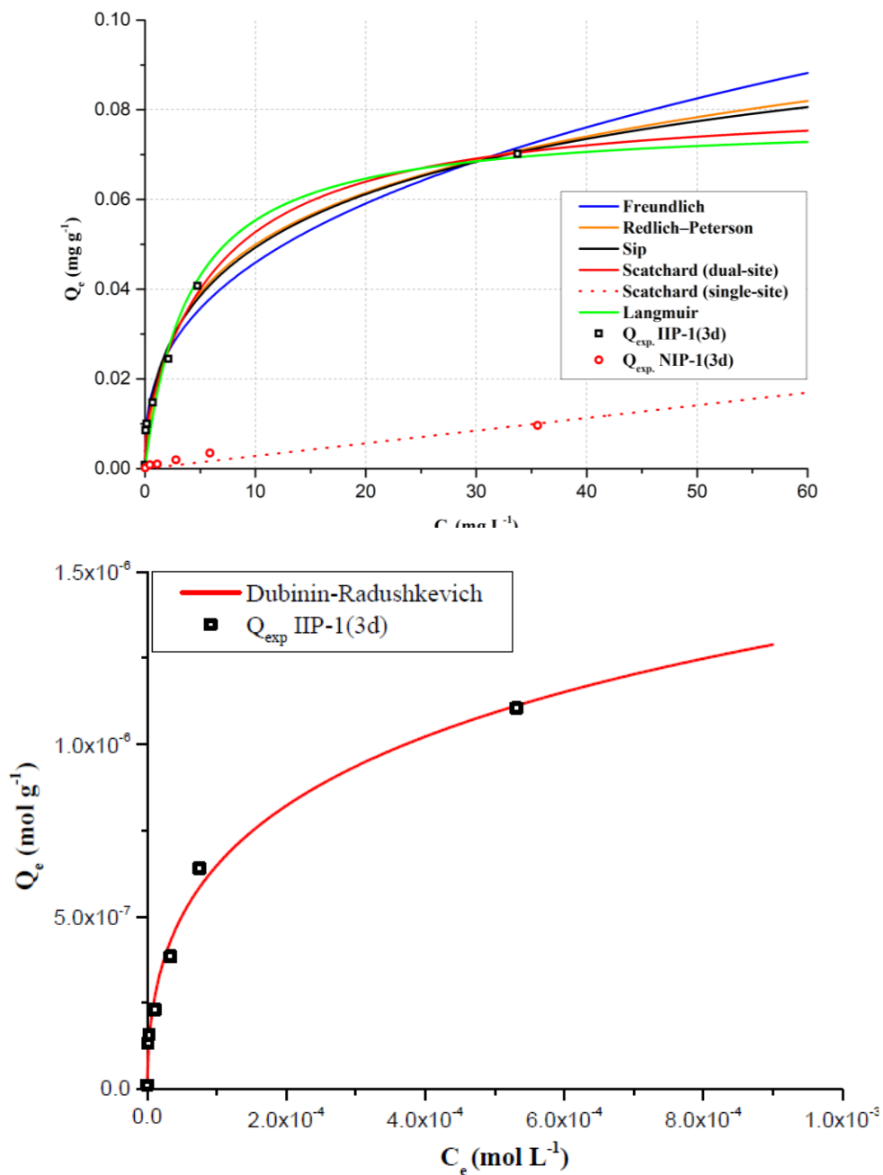
Figure S4: Plots of the isotherm models with the experimental data of IIP-1(3d) and its NIP.
