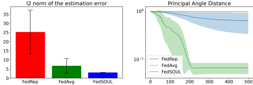
Figure 2: Small data sets - synthetic data.
