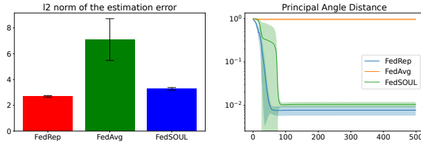
Figure S5: Small data sets - synthetic data. Latent space dimensionality is d = 5 .
