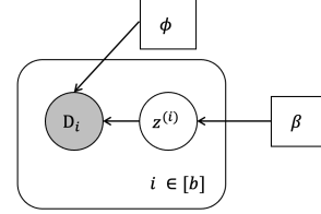
Figure 1: DAG for FedPop.
