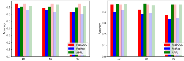
Figure S7: Small image datasets. Minimal local dataset size is 2 (top) or 5 (bottom).
