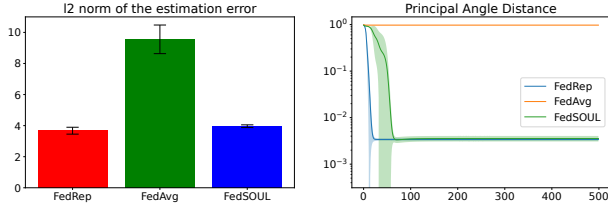
Figure S1: Small data sets - synthetic data. b = 50 clients.
