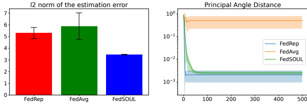
Figure S3: Small data sets - synthetic data. Raw data dimensionality is k = 50 .
