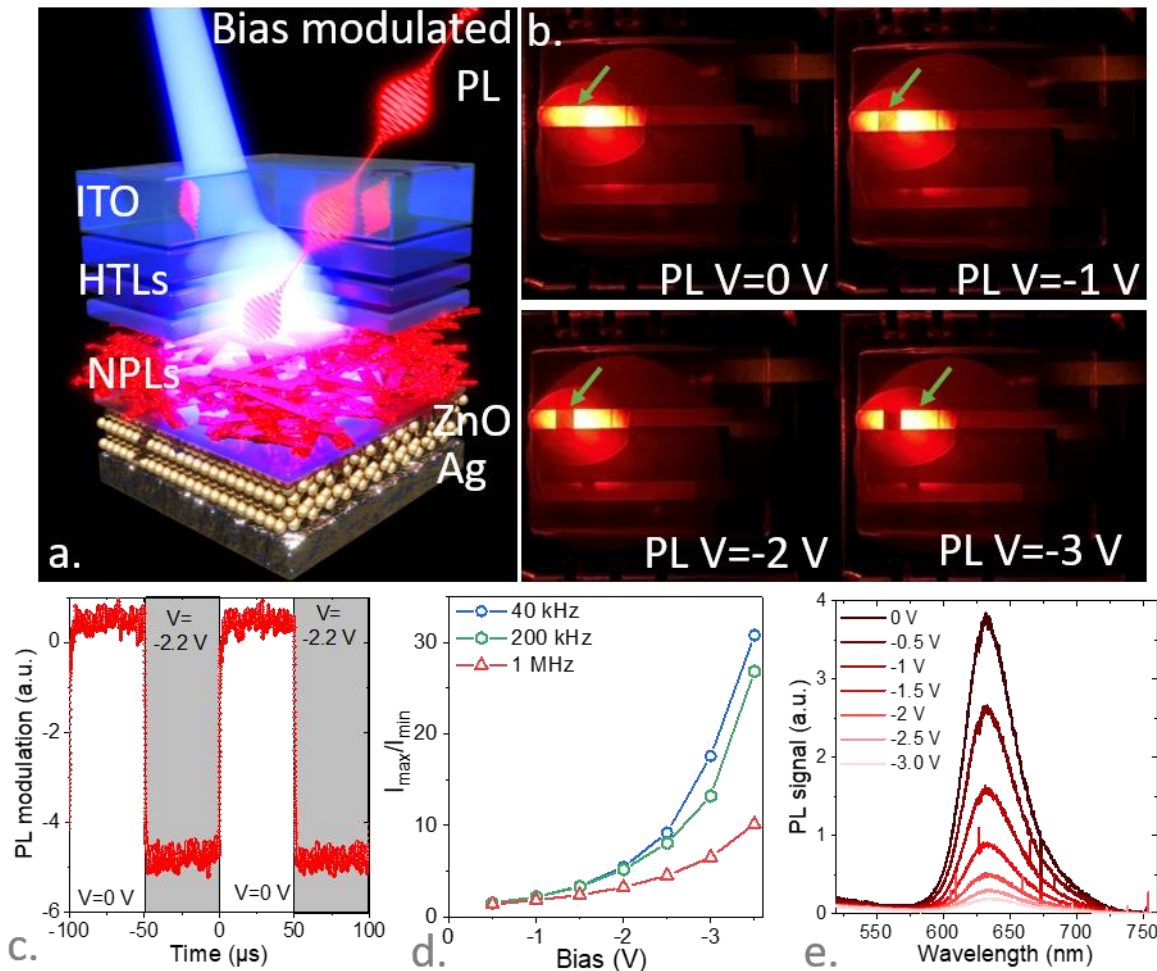
Figure 2. LED stack used as a light modulator. (a) schematic of the LED stack used to modulate the PL magnitude. (b) Images of the NPL-based LED stack under illumination by a blue laser, while various reverse bias voltages are applied on the pixel highlighted by an arrow. The larger the applied reverse bias, the weaker the PL signal from this area. (c) Change in the PL signal resulting from the application of a negative bias pulse as a function of time. (d) Modulation of the PL amplitude (ratio of the signal with and without bias) as a function of the applied reverse bias for various frequency modulations. (e) PL spectra, coming from the pixel area, under various applied reverse biases. Also see Figure S4 for normalized spectra.
