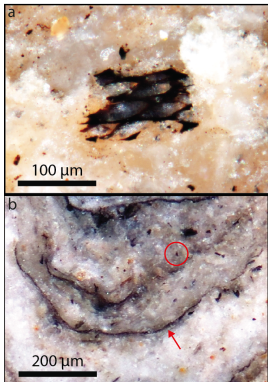
Figure 14. Speleothems found in occupation soils (J and E/F) of the Mandrin cave. (a) Micro-charcoal. (b) Sooty layer (red arrow) and micro-charcs (red circle).
