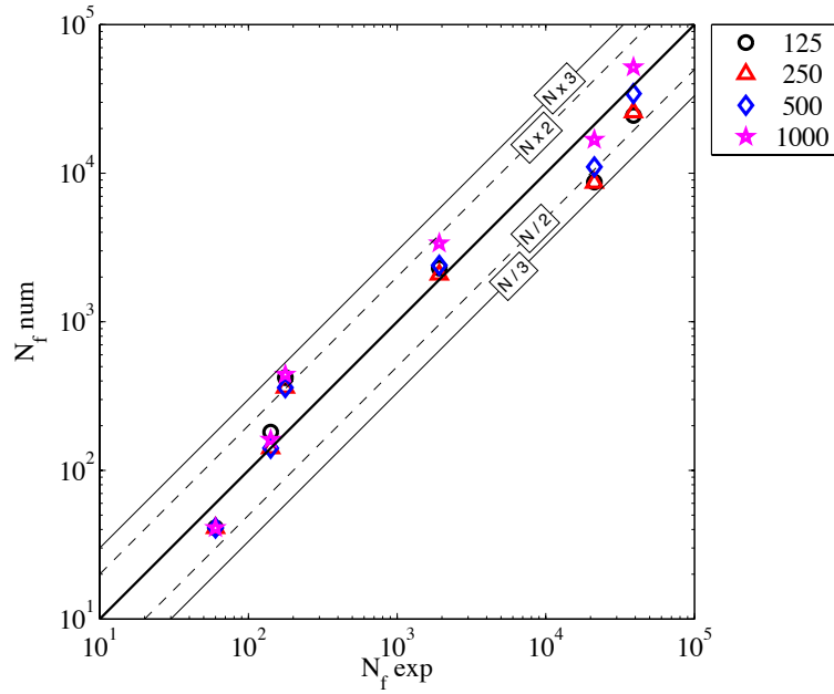
Figure 19: Comparison between the modeled ( N_f^{\text{num}} ) and the experimental ( N_f^{\text{exp}} ) number of cycles to reach a_f as a function of the box size for three holes specimens; the legend indicates the characteristic length of the box size given in \mu\text{m} ; dashed lines and thin lines correspond respectively to a factor of two and three above and below experimental observation
