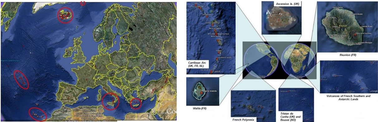
Figure 3. Geographical Distribution of European volcanic areas (red circles) and volcanoes (red triangles) included in EPOS VO-TCS: on the European continent and the Canary Islands (left) and in overseas countries (right).
