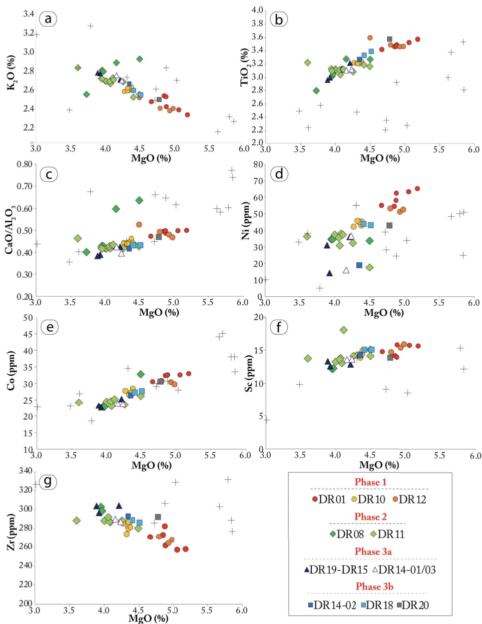
Figure 7. Bulk-rock geochemical evolution of dredged lavas from the eruption site. The caption presents dredges in chronological order. Crosses are reference data for Mayotte lavas [Nougier et al., 1986, Späth et al., 1996, Pelleter et al., 2014].
