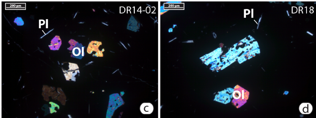
Figure 5. Petrographic characteristics of Phase 3 samples from the NW eruptive site viewed under cross-polarized transmitted light (a) typical olivine crystals in sample DR15. (b) Zoned olivine antecryst in sample DR15 with possible dissolution texture. (c) Sample DR14-02 and (d) sample DR18-01 contain plagioclase laths in the matrix. Ol: olivine, Pl: Plagioclase.
