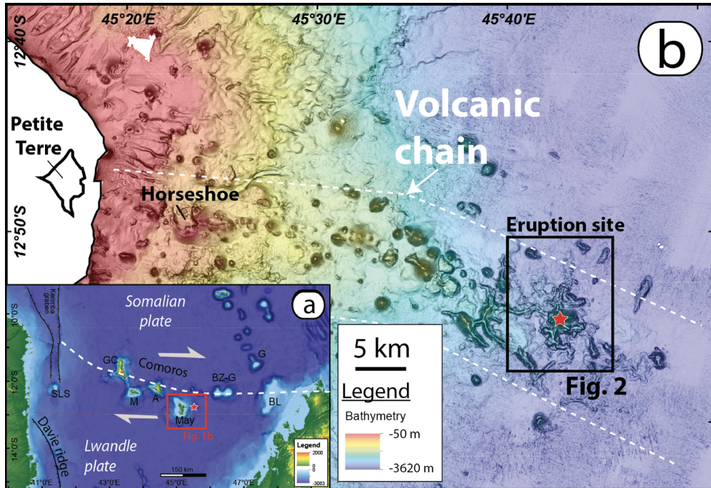
Figure 1. Location of the eruptive site off Mayotte's coast. (a) Comoros Archipelago, underlining the NW–SE boundary between the Lwandle microplate and the Somalia plate from Famin et al. [2020] (white dashed line), is composed of two emerged banks (Zelée and Geyser banks) four main volcanic islands, from east to west, Mayotte (May), Anjouan (A), Moheli (M) and Grande Comore (GC). Red star: eruptive site, G: Glorieuses; BL: Leven Bank; SLS: St Lazarus Seamount. (b) Fani Maoré volcanic cone is located 50 km east from offshore Mayotte Island, at the end of the Eastern Volcanic Chain, as delineated by the white dashed lines [Bachèlery et al. , 2021, Feuillet et al. , 2021].
