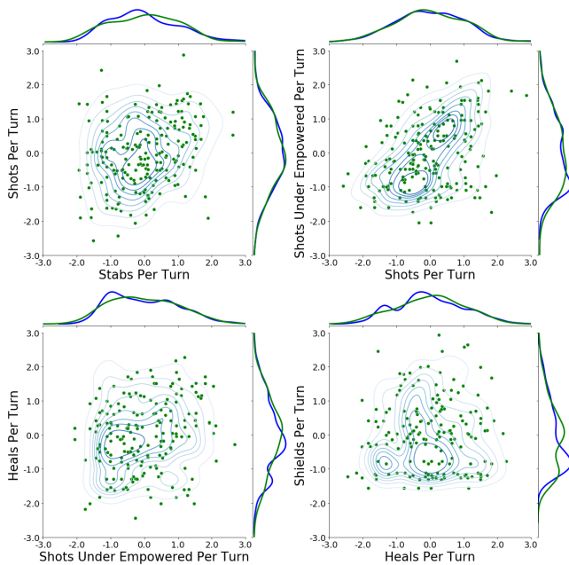
Figure 3: Distribution over the play-modes of players (in green) and CARMI (in blue) normalized summary data, following the sampling strategy described in section 5.2
