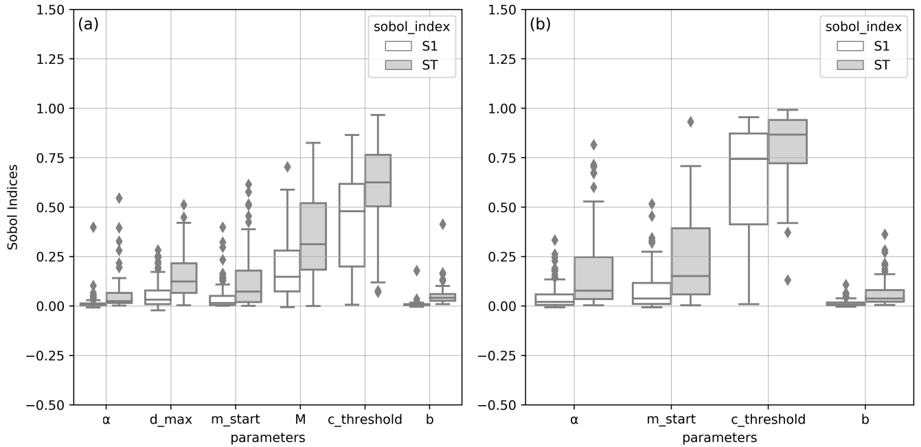
Figure 9. Distribution of first (S1)- and total (ST)-order Sobol indices on the modeled reservoirs for each parameter : (a) in irrigation and (b) in non-irrigation reservoirs
