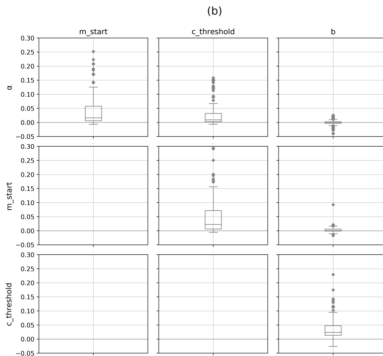
Figure 10. Distribution of second-order Sobol indices (S2) in the modeled reservoirs for each pair of parameters : (a) in irrigation and (b) in non-irrigation reservoirs
