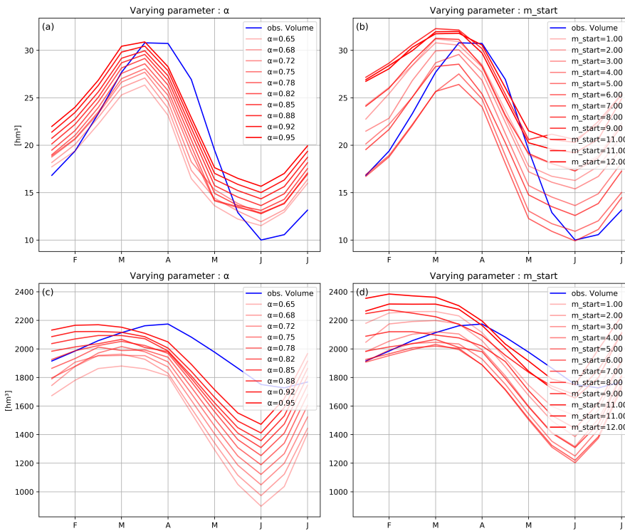
Figure 15. Example of seasonal pattern sensitivity of Gonzalez Lacasa (a,b) and Alcantara II (c,d) reservoir volumes to two of the DROP model parameters : (a,c) \alpha and (b,d) m_{start} . The remaining parameters were set at default values (see Table 2).
