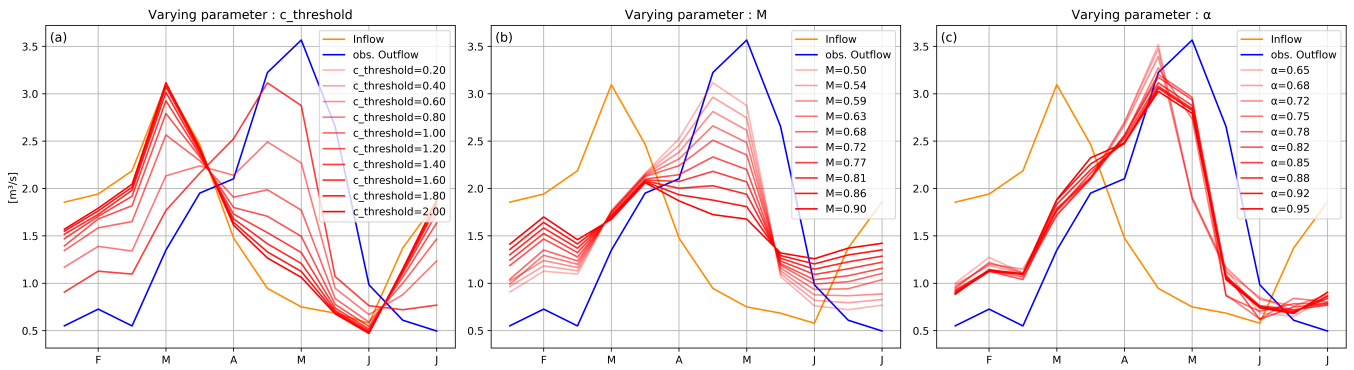
Figure 7. Example of seasonal pattern sensitivity of Gonzalez Lacasa reservoir outflow to three of the DROP model parameters : (a) c_{threshold} , (b) M and (c) \alpha . The remaining parameters were at their default values (see Table 2).
