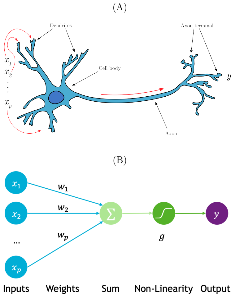
Figure 2: (A) Biological neuron. The synapses form the input of the neuron. Their signals are combined and if the results exceeds a given threshold, the neuron is activated and produces an output signal which is sent through the axon. (B) The perceptron: an artificial neuron which is inspired by biology. It is composed of the set of inputs (which correspond to the information entering the synapses) x_i , which are linearly combined with weights w_i and then go through a non-linear function g to produce an output y . Image in panel (A) is courtesy of Thibault Rolland.
