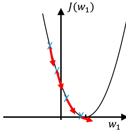
Figure 12: Illustration of the concept of gradient descent in a simple case where the model f is defined using only one parameter w_1 . The value of w_1 is iteratively updated by following the opposite of the gradient.
