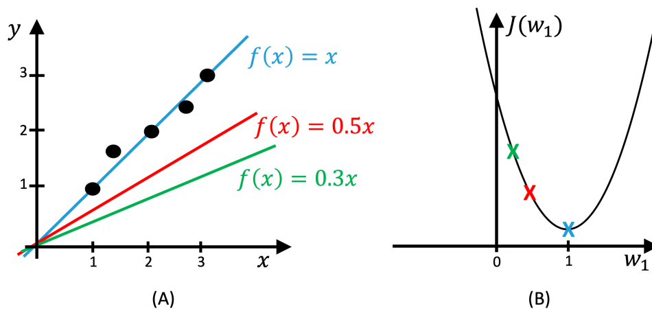
Figure 11: We illustrate the concepts of supervised learning on a very simple case: univariate linear regression with no intercept. Training samples correspond to the black circles. The different models f(x) = w_1x correspond to the different lines. Each model (and thus each value of the parameter w_1 ) corresponds to a value of the cost J(w_1) . The best model (the blue line) is the one which minimizes J(w_1) , here it corresponds to the line with a slope w_1 = 1 .
