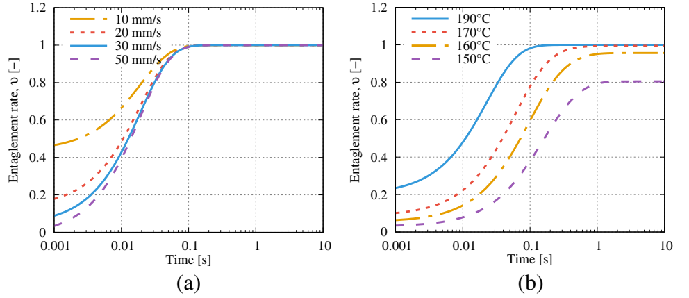
Fig. 6 Example of entanglement rate evolution after filament deposition for a different printing speed at 190 °C and b different extrusion temperatures with U_N = 30\text{mm/s}
