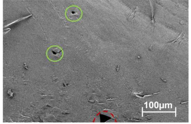
Fig. 11 Scanning electron micrographs of cross sections taken in bulk specimens of neat PDLLA
