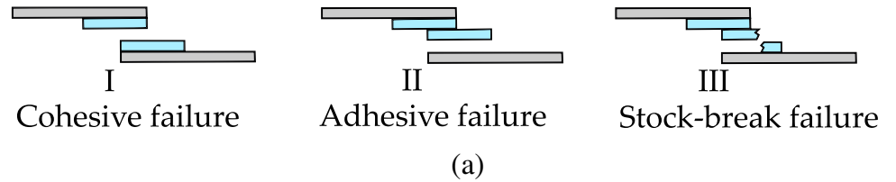
Fig. 12 a Representation of lap-shear system and the different failures modes observed in the tests and b experimental results from lap-shear test ( \sigma_{\text{weld}}/\sigma_{\text{bulk}} ) vs model prediction ( (t_h/\tau_w)^{1/4} ) for PDLA, purple square represents the zone with a stock-break failure
