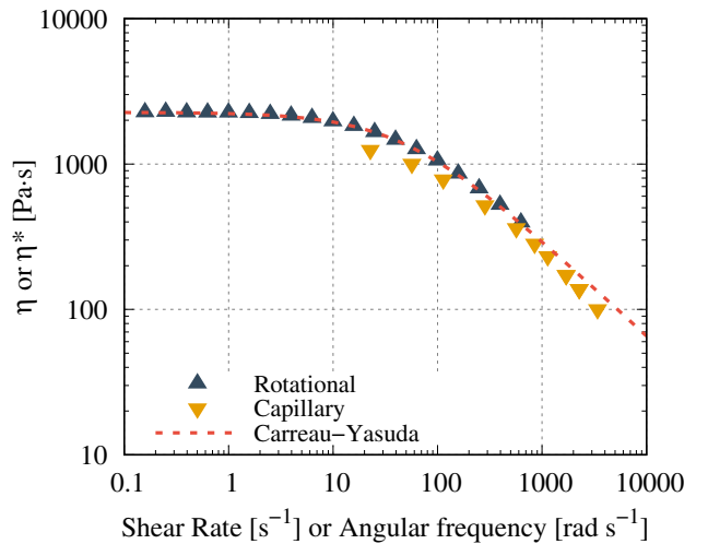
Fig. 4 Complex viscosity modulus (rotational) and corrected shear viscosity (capillary) respectively as a function of angular frequency and real shear rate for PDLLA at 190 \text{ }^\circ\text{C}
