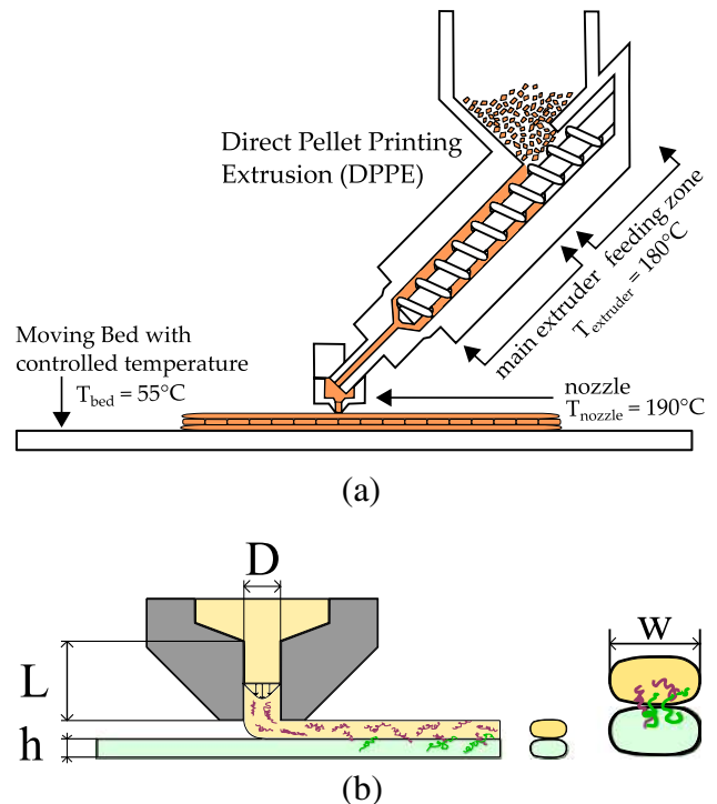
Fig. 1 a Schematic representation of the DPPE process. b Schematic representation of the deposition process and welding of filaments, highlighting chains interdiffusion with deposition time. D and L are respectively 0.4 \text{ mm} and 2 \text{ mm}
