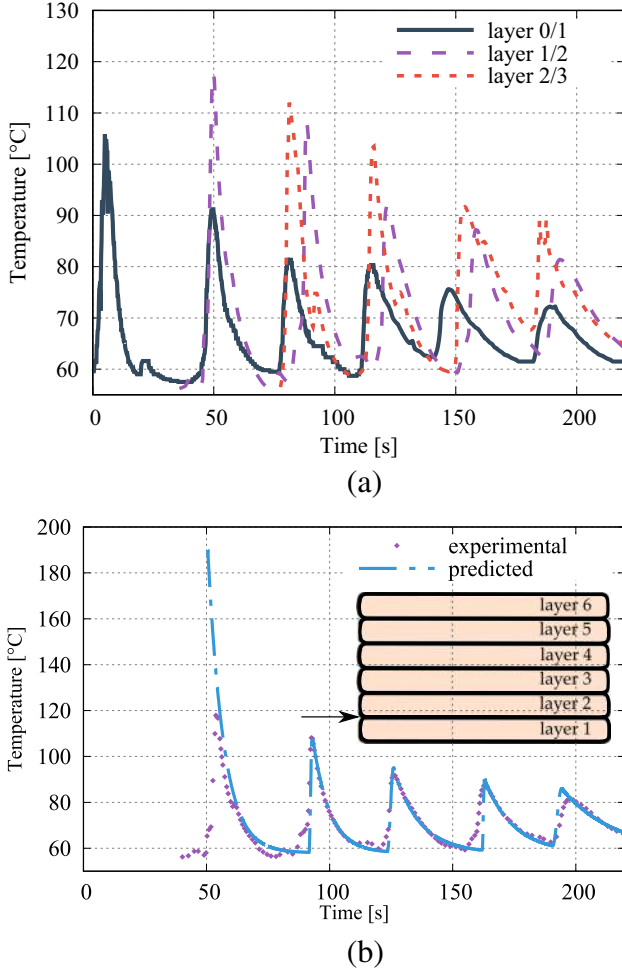
Fig. 3 a Temperature evolution of different interfaces and b experimental and modeled temperature evolution of the interface between layer 1 and 2 during printing at T_{\text{ext}} = 190 \text{ }^\circ\text{C} and V_{\text{imp}} = 30 \text{ mm/s} for a tensile sample as a function of printing time
