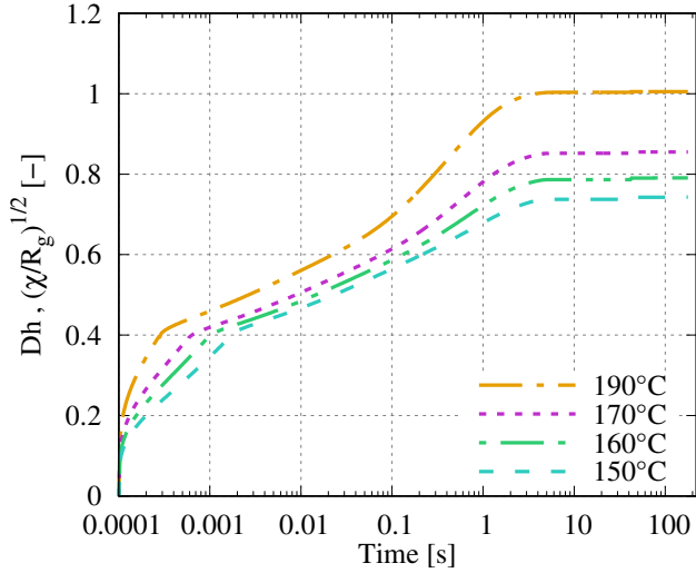
Fig. 10 Evolution of healing degree D_h after deposition calculated from the interphase thickness for PDLA at different printing temperatures for the interphase between layers 1 and 2
