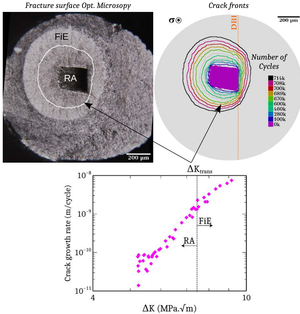
Figure 10: Example of quantitative analysis of crack growth rates within the RA and the FiE region for sample C2. The transition between the two region is determined by combining optical inspection of the fracture surface and 3D crack fronts obtained from tomography. For this sample the transition occurs at \Delta K_{\text{trans.RA} \rightarrow \text{FiE}} .
