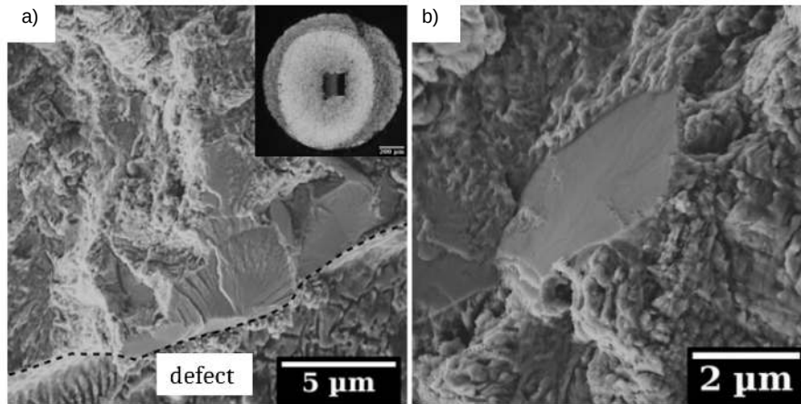
Figure 9: (a) Fracture surface of a sample with an internal defect; the granular region ahead of the facets corresponding to crack initiation is typical of crack propagating in vacuum b) Magnified view of a facet surrounded by granular region.
