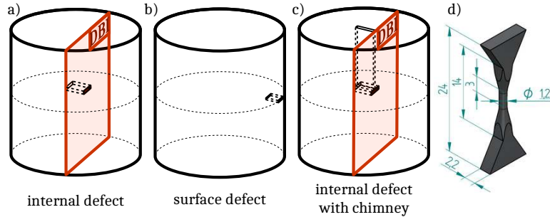
Figure 1: Schematic drawing of the different location of defects within the fatigue specimens used for in situ and ex situ tests. a), b), c) enlargement of the central gauge length, d) geometry and size of the specimens.
