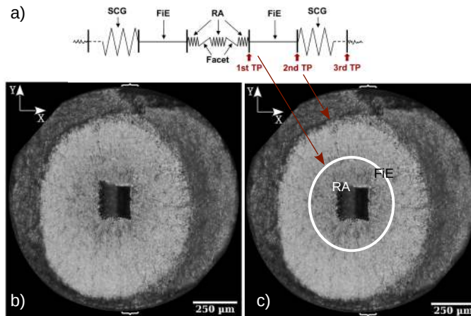
Figure 6: a) Schematic description of the different regions surrounding the crack initiation site (natural crack) in a Ti alloy as proposed by Hong and Sun [8]. b) and c) typical optical micrographs showing the initiating notch in the center, the Rough Area (RA) and the Fish Eye (FiE) regions.
