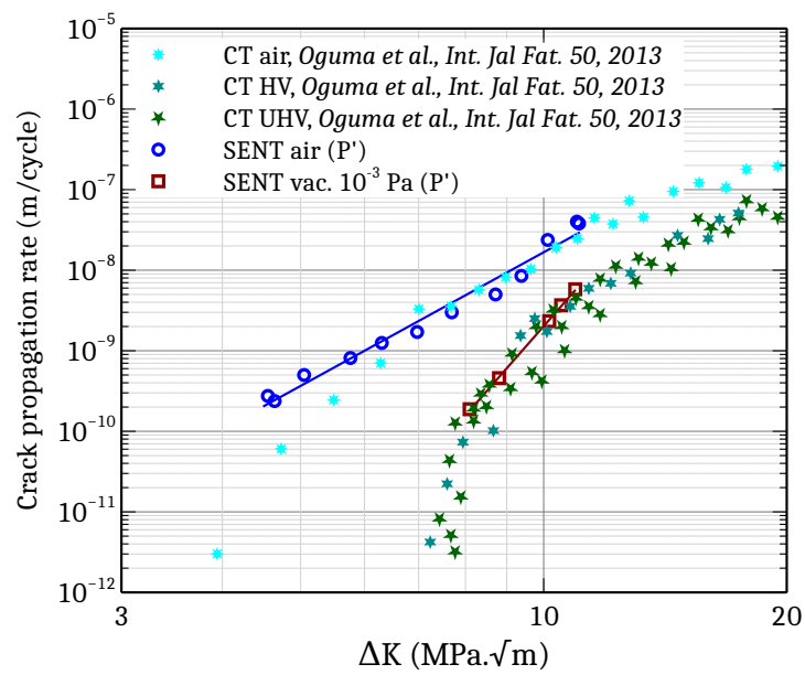
Figure 3: Crack propagation curves obtained by SENT tests on the Ti sheets in vacuum and in air. Prior to testing the sheets have been submitted to a heat treatment corresponding to the welding cycle in the SPS.
