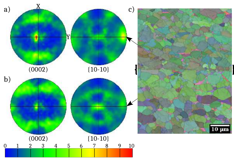
Figure 2: EBSD maps of the microstructure of the two different sheets used after diffusion bonding. The bonding interface is indicated by the {} symbols. The texture is similar in both sheets with a slightly larger number of basal planes perpendicular to the rolling direction (the loading direction of the fatigue tests) in the sheets where the laser notch is machined.
