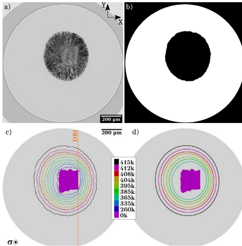
Figure B.12: Tomographic image processing procedure. a) Projected image of the crack of specimen A3 at 400 kcycles. b) Corresponding segmentation. c) Superposition of all crack fronts observed for specimen A3. d) fitted ellipses.
