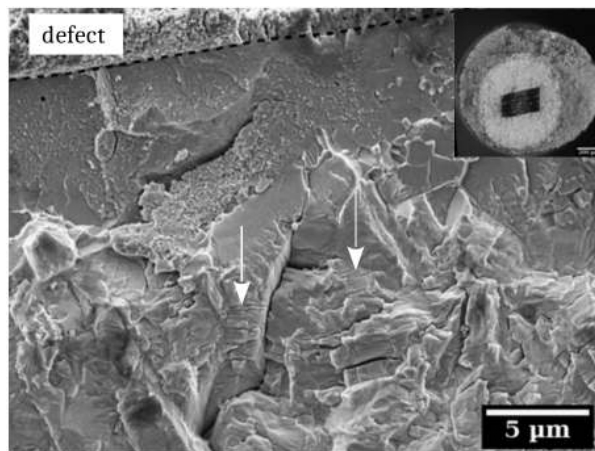
Figure 8: Fracture surface of a sample with a chimney. The arrows point at marks which could be striations typical of crack propagation in air.
