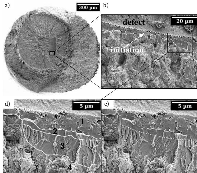
Figure 7: Fractography of sample C2. a) Global view. b) Zoom on the crack initiation site. c) and d) Zoom on the initiation region showing the evolution of the fracture surface from some cleavage facets at the edge of the artificial defect (zone 1) to a rough morphology characteristic of propagation under vacuum (zone 4) with a transition zone in between (zone 2 and 3) with some quasi
