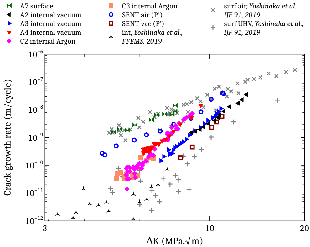
Figure 5: Propagation curves obtained with the samples with artificial defects, compared with literature data and with the SENT tests performed in this work.
