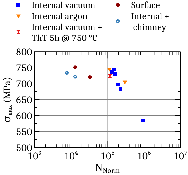
Figure 4: S-N curves obtained from the ex situ fatigue tests. The numbers of cycles to failure are normalised by the fatigue life of the sample with the smallest artificial defect as explained in Appendix A
