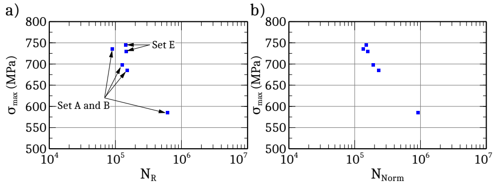
Figure A.11: S-N curves for the ex situ fatigue tests: a) without normalization and b) with normalization by the initial defect size (equation A.3). Three sets of plates (A, B and E) were used to produce the specimens. The notch sizes were similar in A and B and slightly larger than in E
