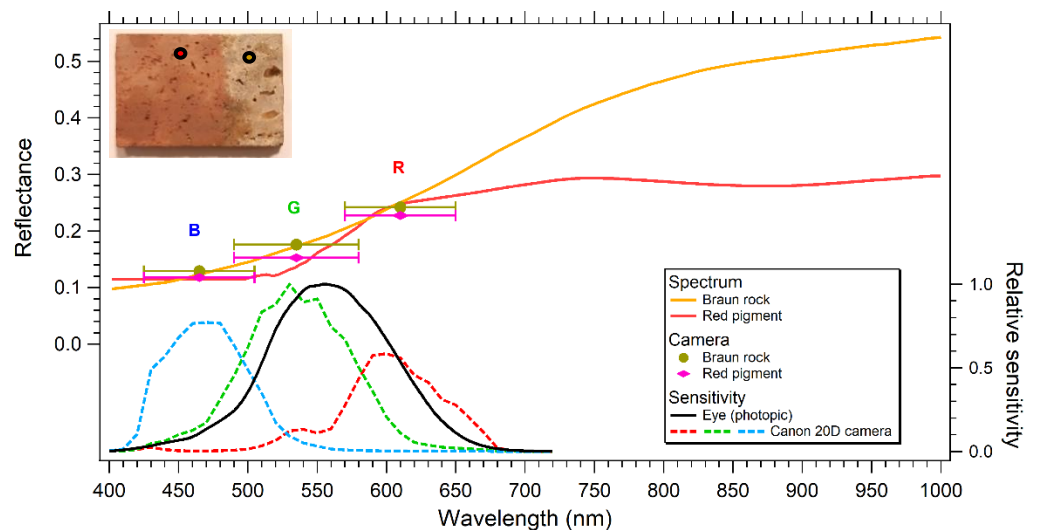
Fig. 2. Comparison between spectra of VNIR hyperspectral imaging and signal of classical RGB camera for typical rock painting pigments. The high-resolution reflectance spectra measured on a very thin layer of red 'Beauregard' pigment (red) painted on a carbonate rock, and the non-painted rock itself (brown) are plotted with a continuous line (left scale) [50]. The large dots are simulations corresponding to the RGB signal of a digital camera (Canon 20D, [31]) extracted from these spectra by convolving them with its filter band passes (dotted lines at the bottom, right scale) with 'error bars' representing the full width at half maximum of the three filters. The bottom black curve is the total photopic eye sensitivity [26].
