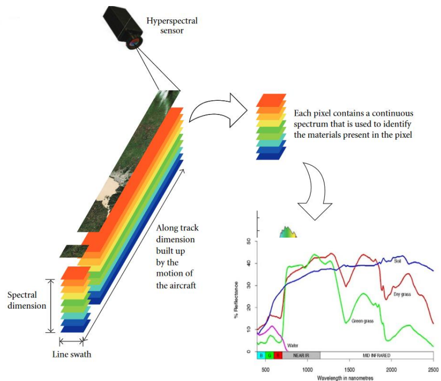
Fig. 1. In a hyperspectral imaging's pushbroom mode, the camera scans the surface line by line and record a full spectrum at each pixel location. An image at each wavelength forming a 3D data cube is obtained (Two spatial dimensions and one in the spectral dimension) (adapted from [34]).
