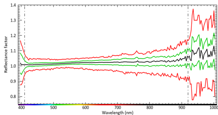
Fig. 5. Statistics on the spectra of the reference target (~2700 pixels) with mean (black), mean +/- standard deviation (green), min and max values (red) showing the increasing noise below 410 nm and above 920 nm. Only the central part of the spectrum (dashed lines: 410-920 nm) with standard deviation < 5% is kept for the hyperspectral data analysis.
