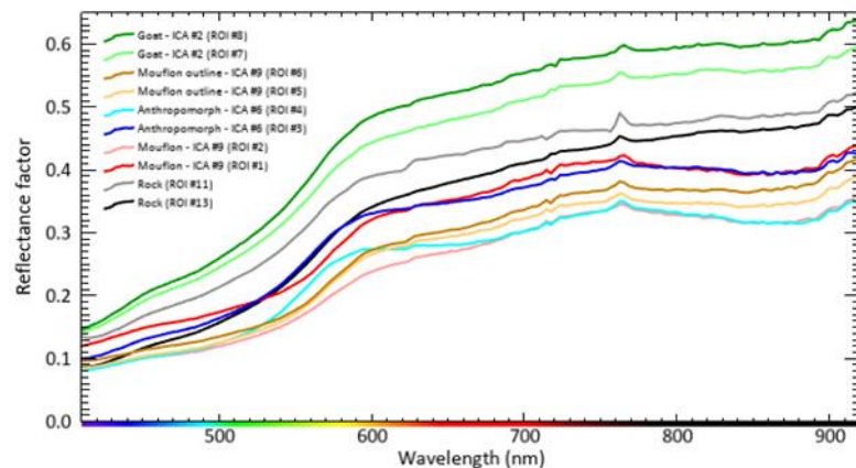
Fig. 20. End-member spectra (average of 35 to 75 pixels for pigments, > 300 for rock) of the Barbary sheep pigment (light and dark red) and its outline (orange and brown), the anthropomorph pigment (dark and light blue), the goat (light and dark green) and typical rock wall area (grey and black) selected in the hyperspectral image of panel #4 presented in Fig. 17.
