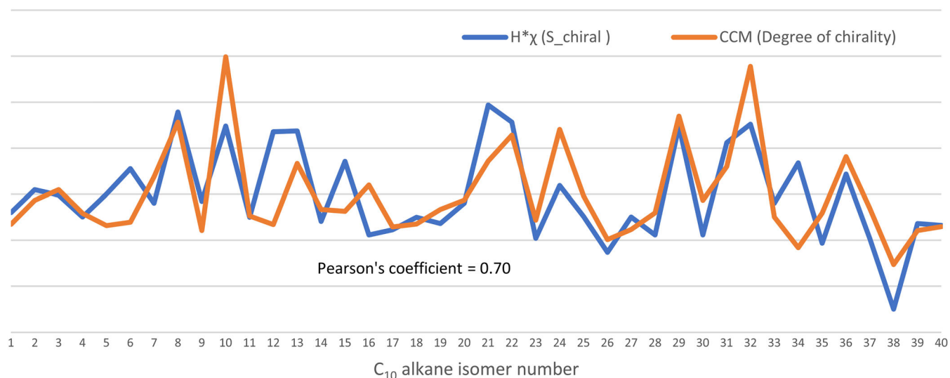
FIGURE 16 Comparison of the normalized distributions of H_{\chi}^*(S_{chiral}) and the CCM degree of chirality of 3D-optimized chiral C_{10} alkane isomers. Isomers are ranked on the x-axis according to Table 1 numbering
