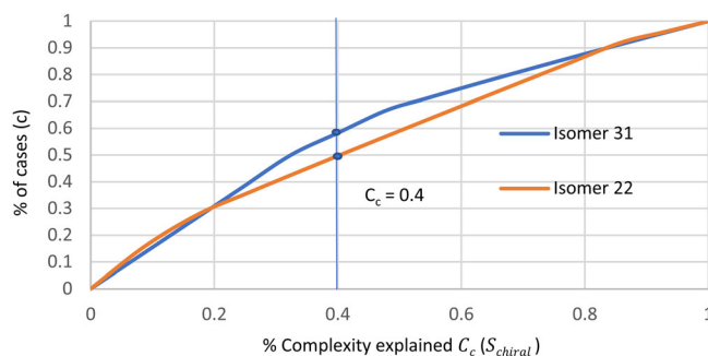
FIGURE 11 Diversity contribution C_c versus the cumulative frequency of cases c of S_{chiral} for isomers 31 and 22. The two isomers 31 and 22 have a similarly high level of chiral information diversity ( R_{chiral} respectively equal to 0.84 and 0.88), but distribution of complexity C_c of isomer 31 is more restricted than isomer 22
