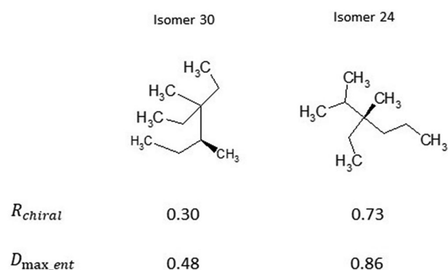
FIGURE 8 Comparison of two C_{10} alkane isomers in term of chiral information richness ( R_{chiral} ). Chiral complexity of isomer 30 is less important, that is, contains less diversity around the chiral center than isomer 24
