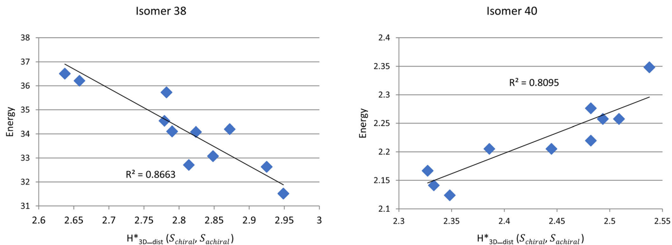
FIGURE 15 3D distance-based joint entropy versus conformation energy of alkane isomers 38 and 40
