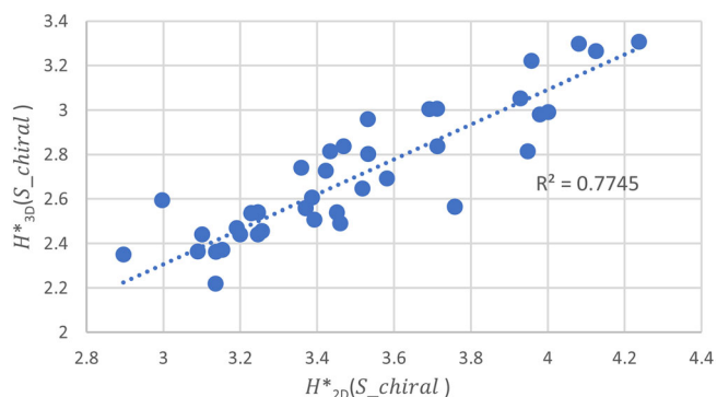
FIGURE 13 Relationship between H_{2D}^*(S_{chiral}) and H_{3D}^*(S_{chiral})
