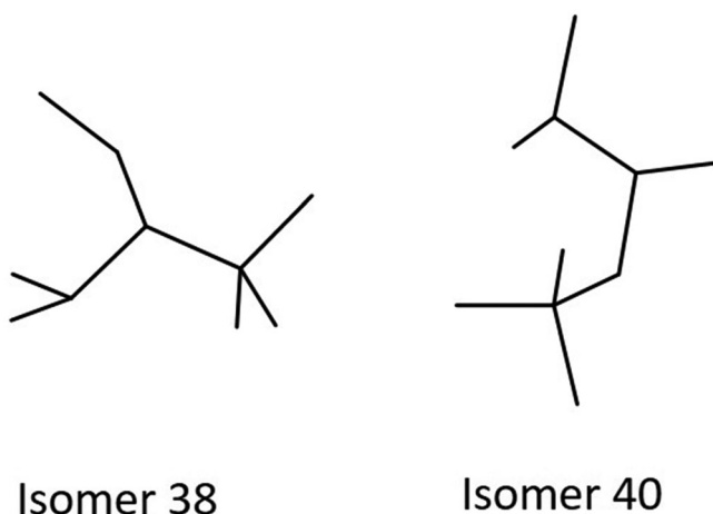
FIGURE 14 Lowest-energy conformation of alkane isomers 38 and 40. Isomer 38 presents a higher geometrical distance diversity than isomer 40 which contains more symmetries in the spatial arrangement
