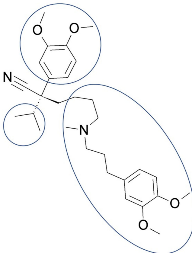
FIGURE 2 Example of “achiral portions” that can be isolated in a chiral molecule. Any atom pairs randomly selected in these regions have no stereogenic element in their shortest path
