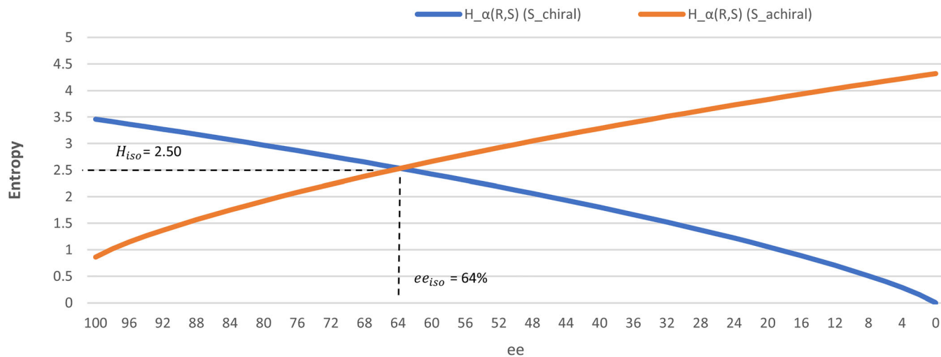
FIGURE 18 Common graph of the evolution of H_{\alpha(R,S)}(S_{chiral}) and H_{\alpha(R,S)}(S_{achiral}) versus the ee (example shown is 3D-optimized isomer 18)
