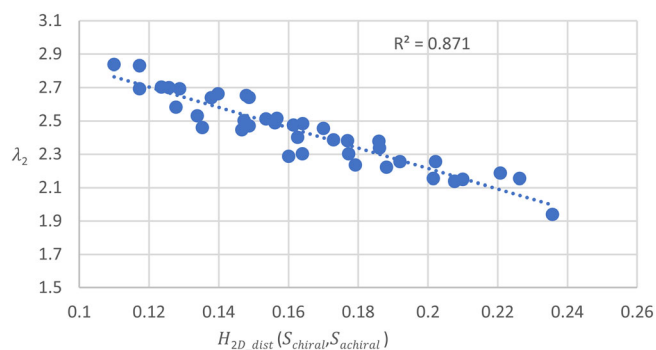
FIGURE 6 Correlation between eigenvalue \lambda_2 and the distance-based joint entropy H_{2D\_dist}^*(S_{chiral}, S_{achiral})
