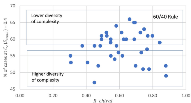
FIGURE 12 Chiral information richness ( R_{chiral} ) versus the cumulative frequency of cases at C_c(S_{chiral}) = 0.4
