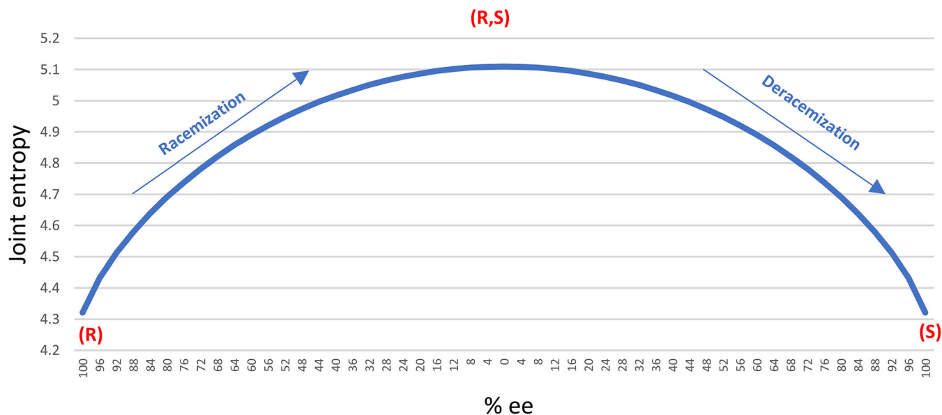
FIGURE 17 Common graph of the evolution of the joint entropy H_{\alpha(R,S)}(S_{chiral}, S_{achiral}) versus the ee (example shown is 3D-optimized isomer 18)
