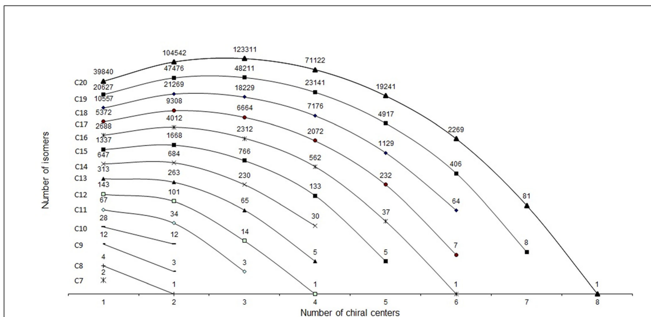
FIGURE 4 Distribution of chiral constitutional isomers of C 7 to C 20 alkanes according to their number of chiral centers (plotted on a log scale)
