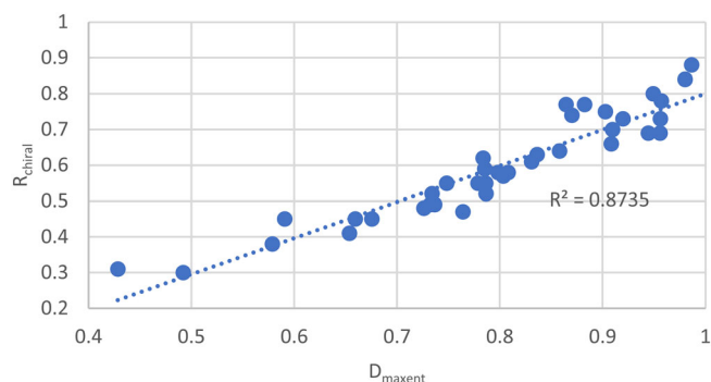
FIGURE 7 Relationship between the chiral information richness R_{chiral} and the distance to maximum chiral entropy D_{maxent}
