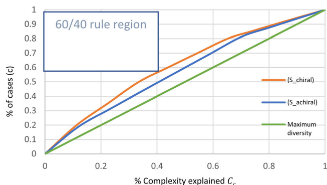
FIGURE 10 Diversity contribution C_c versus the cumulative frequency of cases c (isomer 30, R_{chiral} = 0.30 ). The straight line delineates the theoretical maximum diversity
