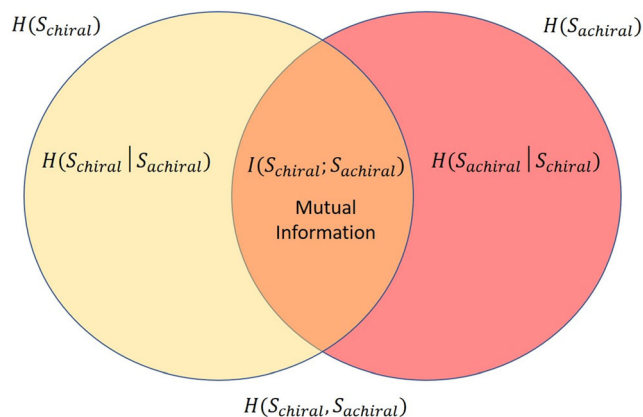
FIGURE 3 Venn diagram of the joint entropy H(S_{chiral}, S_{achiral}) for a chiral molecule in interaction with the environment. The area where both circles overlap is the mutual information I(S_{chiral} : S_{achiral}) of the S_{chiral} and S_{achiral} subset distributions. In case of an isolated molecule, H(S_{chiral}) and H(S_{achiral}) are separated, that is, I(S_{chiral} : S_{achiral}) = 0
