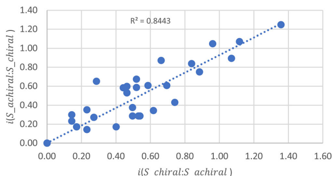
FIGURE 9 Relationship between i(S_{chiral} : S_{achiral}) and i(S_{achiral} : S_{chiral}) contributions to mutual information
