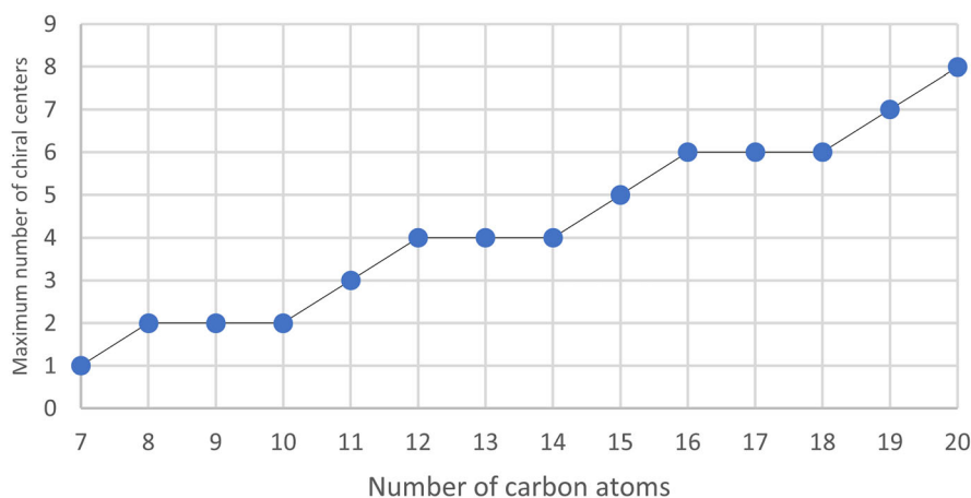
FIGURE 5 Plot of the number of carbon atoms n versus the maximum number of chiral centers that can be found in constitutional isomers of C 7 to C 20 alkanes
