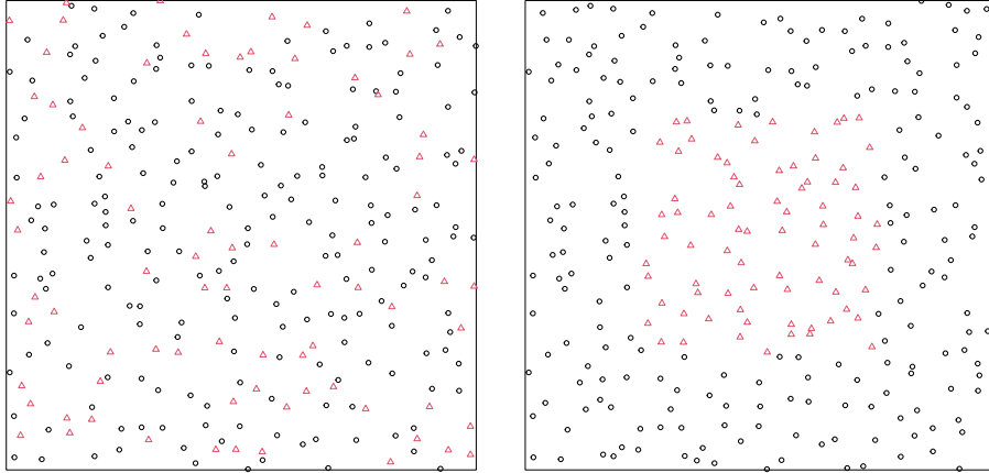
Figure 2: Conditional simulation of the red points (shown as triangles) given the black points, assuming that the full point pattern formed by the union of the black and red points is a projection DPP. Left: simulation in the whole domain. Right: simulation in the inner square (in-painting).
