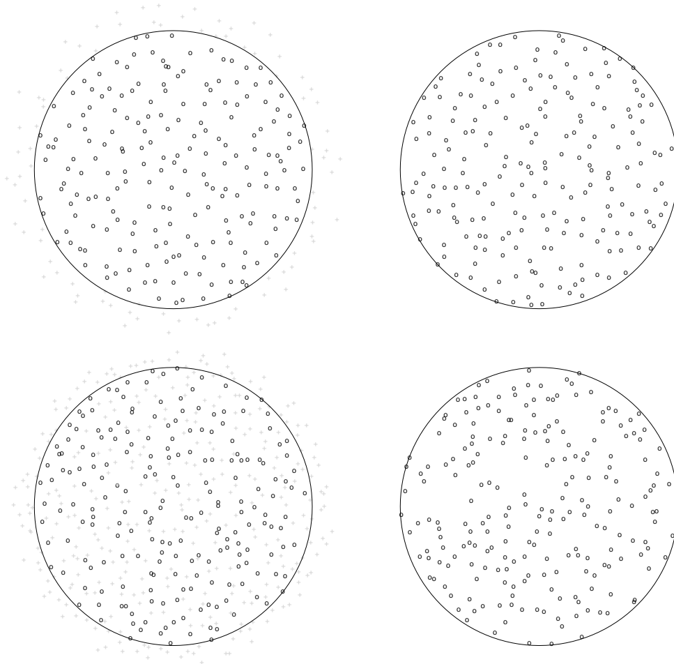
Figure 3: Realisations of two \beta -Ginibre processes generated with Algorithms 4 (left) and 5 (right). In all cases \rho = 200 . In the top row \beta = \beta_{\max} and in the bottom row \beta = \beta_{\max}/2 . For Algorithm 4 on the left the gray points represent the points deleted by the algorithm.
