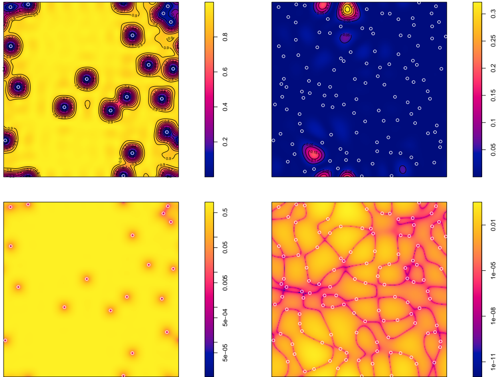
Figure 1: Conditional density p_i at intermediate steps of Algorithms 1 and 2, for the Fourier basis and n = 121 on the unit square. Top row is untransformed values while the bottom row is in log scale. Left: density of the 20th point given the 19 first ones (superimposed as white circles); right: density of the last point given the preceding 120 points.
