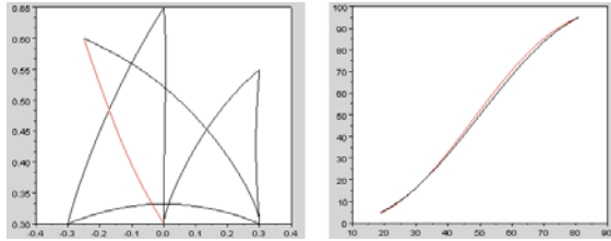
Figure 10: Experiment 3.1 ( simulation ) : (a) - translation part of the global sequence of movements (black) and of the studied movement (red) (b) - Comparison between the time evolution of the hand orientation (red) and the minimum jerk (black).
