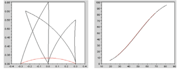
Figure 12: Experiment 3.2 ( simulation ) : (a) - translation part of the global sequence of movements (black) and of the studied movement (red) (b) - Comparison between the time evolution of the hand orientation (red) and the minimum jerk (black).
