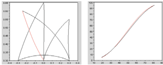
Figure 10: Experiment 3.1 ( simulation ) : (a) - translation part of the global sequence of movements (black) and of the studied movement (red) (b) - Comparison between the time evolution of the hand orientation (red) and the minimum jerk (black).
