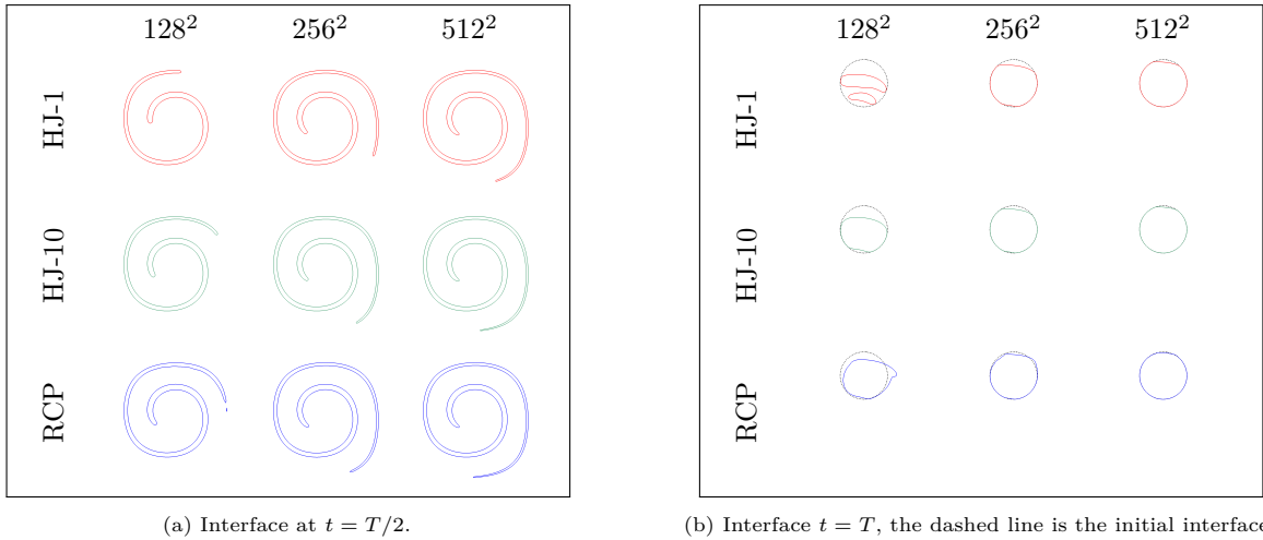
(a) Interface at t = T/2 . (b) Interface t = T , the dashed line is the initial interface. Figure 13: Single vortex 2D test case: interface shapes at t = T/2 (left) and t = T (right).
