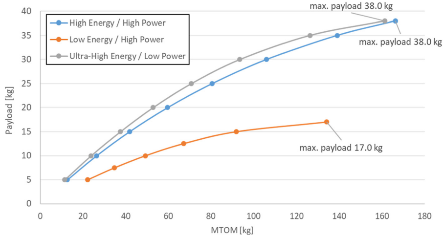
Fig. 10. Payload effect on maximum takeoff mass for three different battery cell types and a fixed range.
