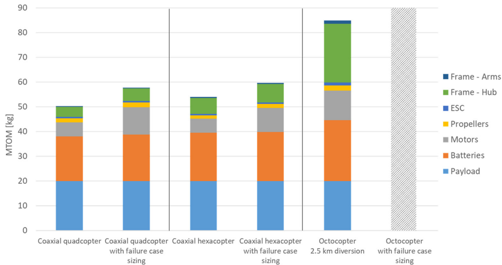
Fig. 9. Mass breakdown results from the preliminary design.
