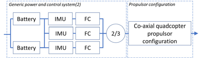
Fig. 7. Coaxial quadcopter propulsion system reliability block diagram (single fault-tolerant architecture).
