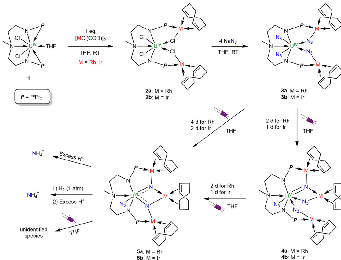
Fig. 2 Synthesis and reactivity of complexes 2 , 3 , 4 , and 5 . Complexes 3a and 3b with four azides were prepared by the reaction of complexes 2 with NaN_3 . By careful control of the irradiation time of complexes 3 , the U(VI) nitrides 5 were formed via the U(V) nitrides intermediates 4 . The nitride groups in complexes 5 react with acid or H_2 /acid to form NH_4^+ in good yield. The N atoms originating from N_3^- are shown in blue and transition metals (M) are shown in red.
