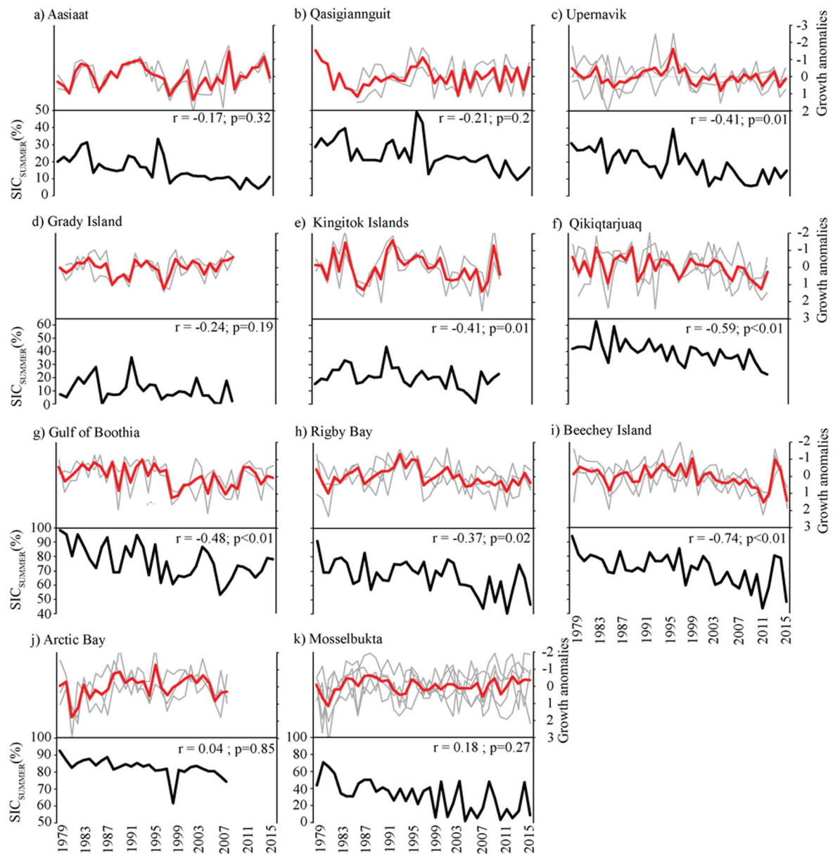
Figure 4. Algal growth anomalies (red) and SIC_{SUMMER} (black: May–October means) time series. Algal growth anomalies from individual samples in gray. Note that algal growth anomalies are presented on inverted axis.
