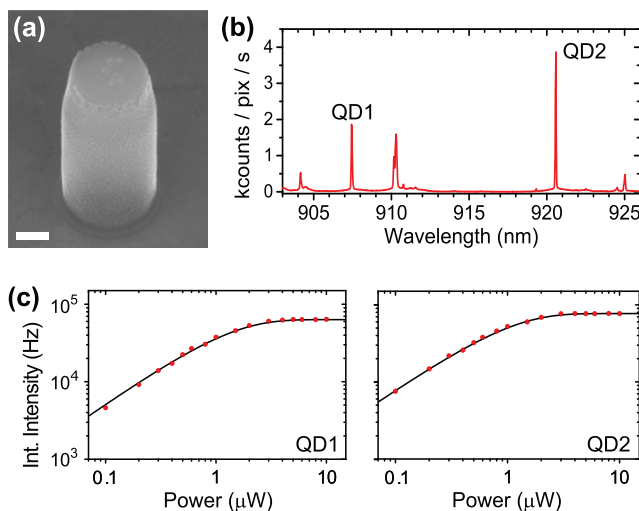
FIG. 2. (a) Scanning electron microscope image of a representative device (tilted view; scale bar, 100 nm). (b) Micro-photoluminescence spectrum as measured on the CCD under pulsed excitation ( P_{exc} = 300 nW) at T = 4 K. (c) Spectrally integrated intensity I of lines QD1 and QD2 as a function of P_{exc} . The dots correspond to experiments and the solid line to theory (see the text for details).
