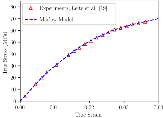
Figure 2: True stress-strain curve obtained experimentally under uniaxial tension and fitted using Marlow model.
