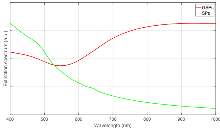
Fig. 2. Extinction spectra of SP and GSP solutions.
